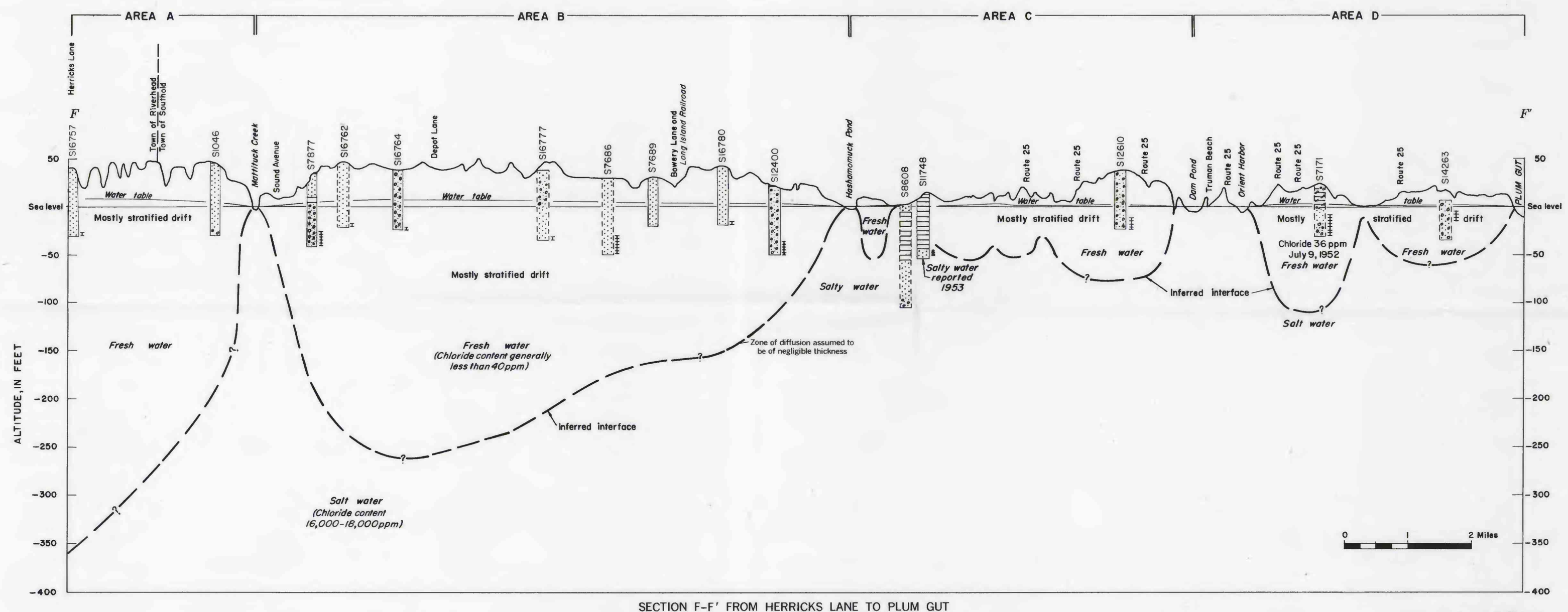
GEOHYDROLOGIC SECTIONS IN THE TOWN OF SOUTHOLD, SUFFOLK COUNTY, NEW YORK
