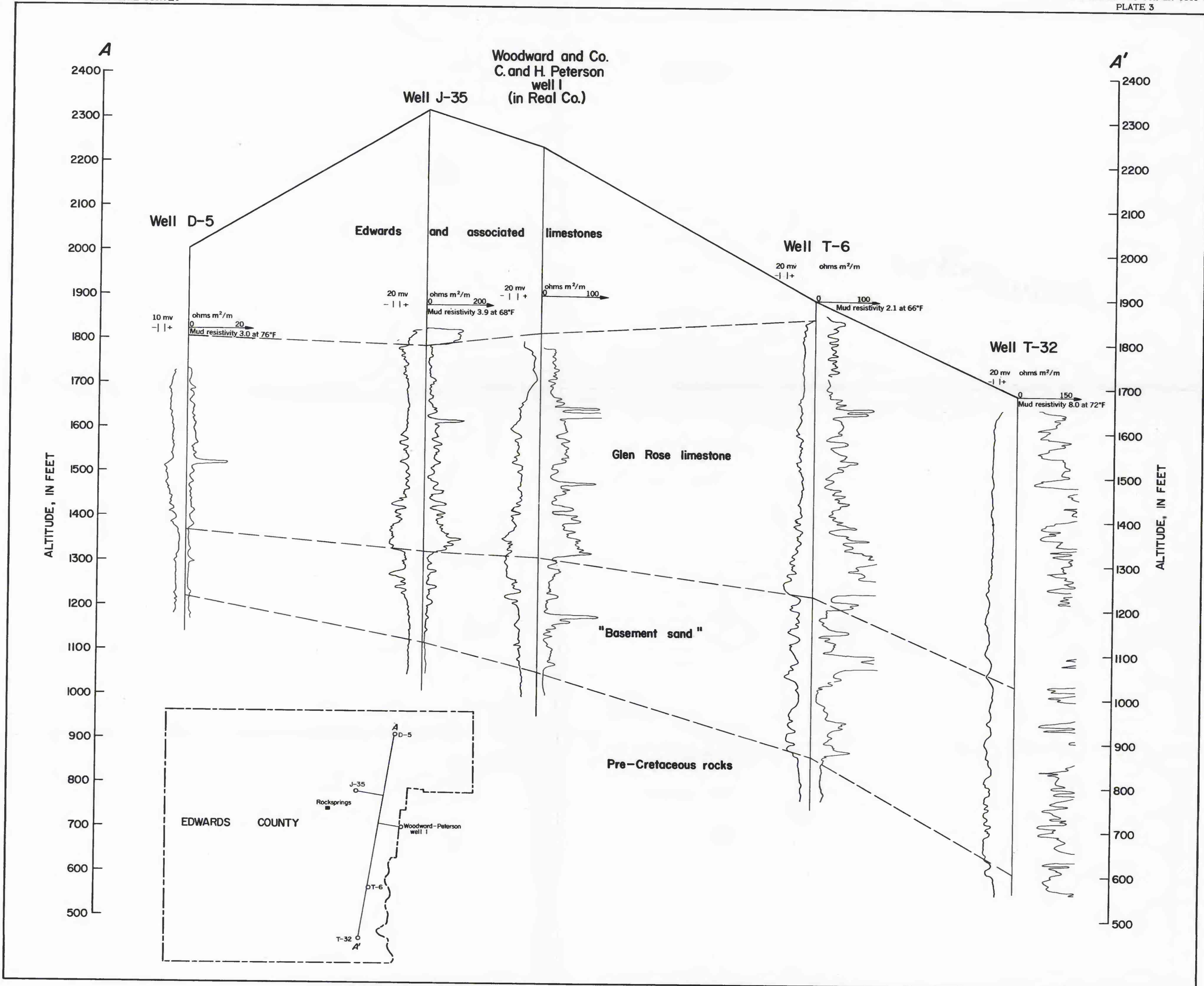
GEOLOGIC SECTION A-A', EDWARDS COUNTY, TEXAS
