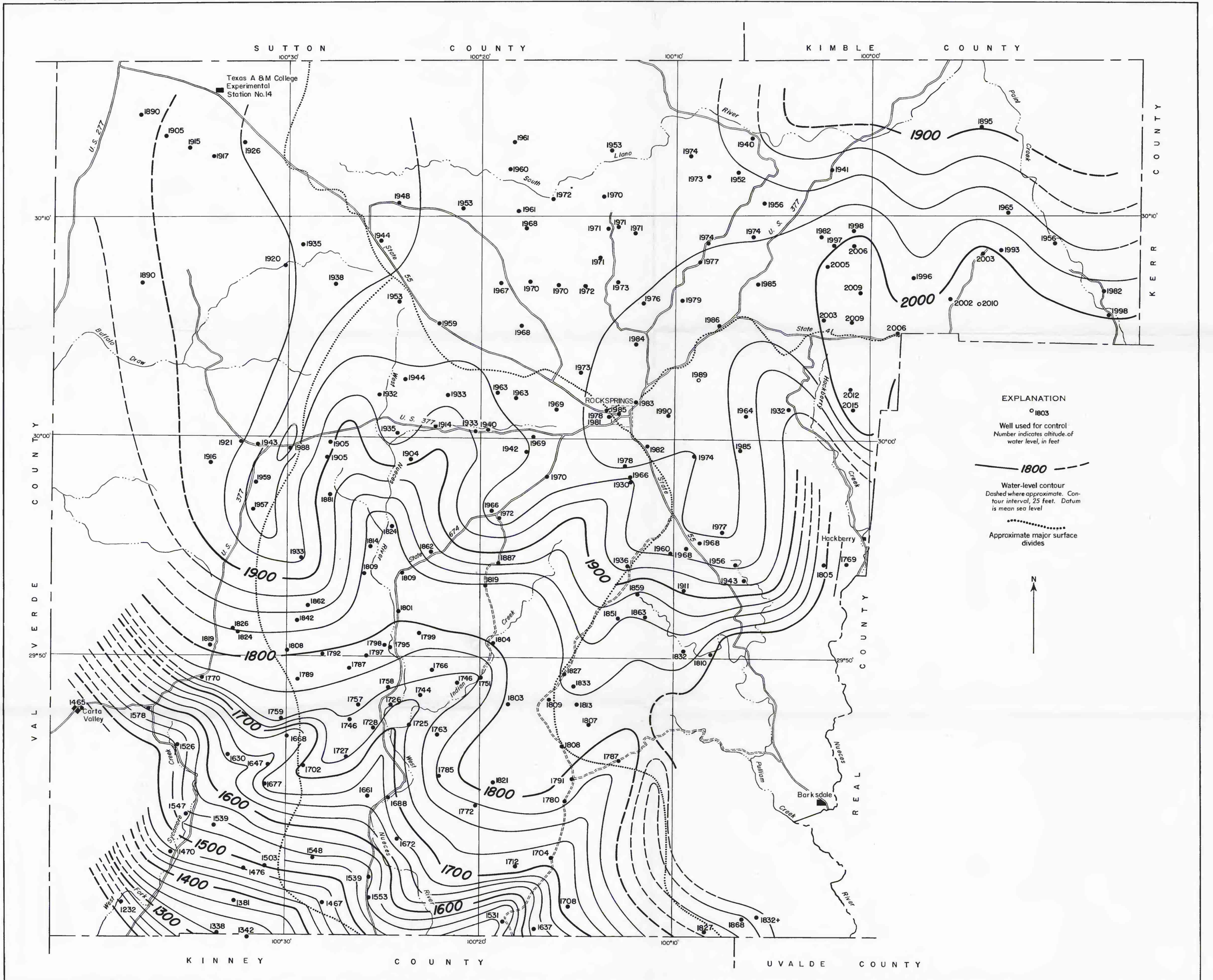
APPROXIMATE ALTITUDE OF WATER LEVELS IN WELLS IN THE EDWARDS AND ASSOCIATED LIMESTONES EDWARDS COUNTY, TEXAS, OCTOBER 1953-SEPTEMBER 1955
