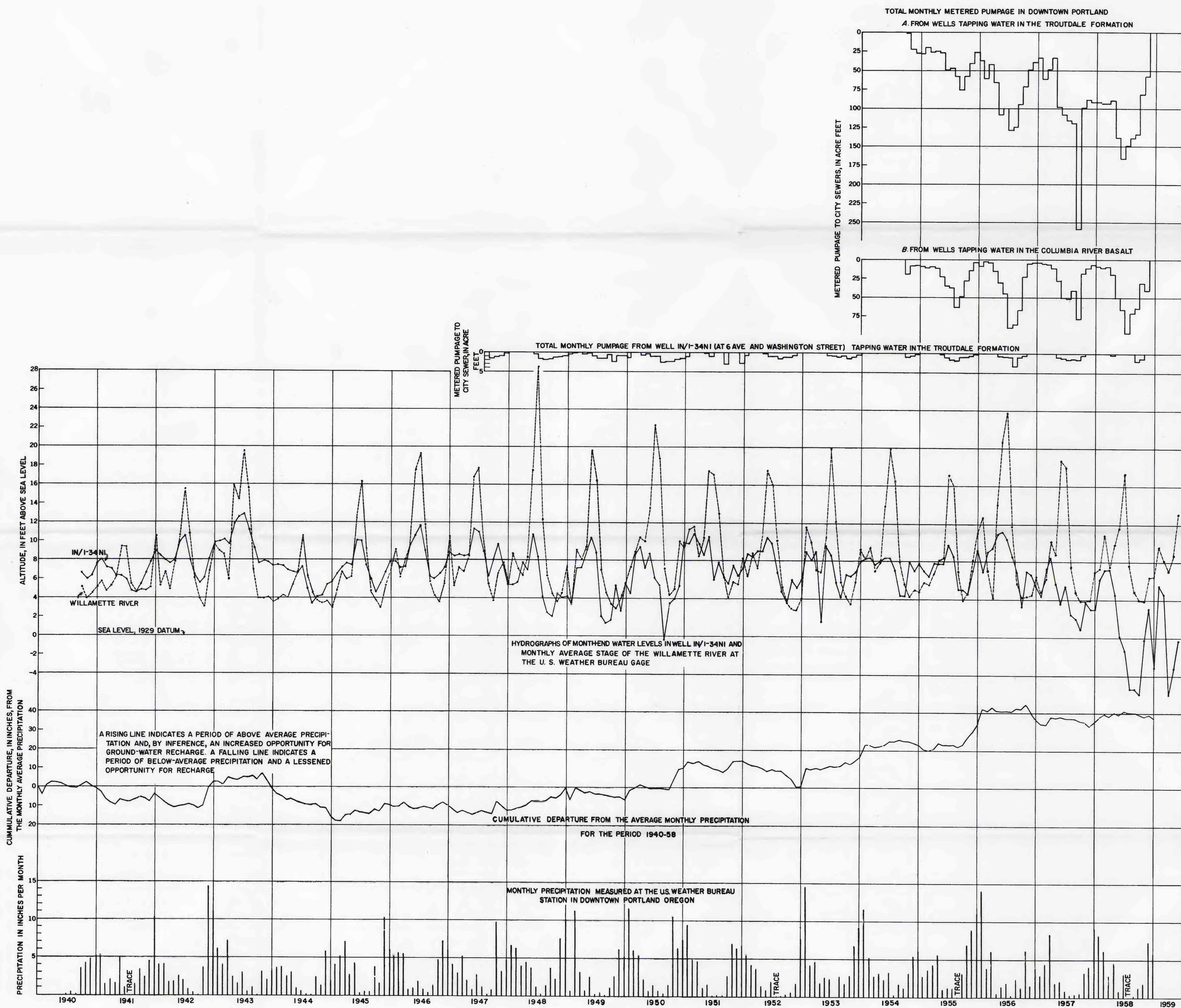
GRAPHS SHOWING WATER LEVELS IN WELL IN/1-34N1, METERED PUMPAGE FROM THAT WELL AND FROM THE TROUTDALE FORMATION AND COLUMBIA RIVER BASALT MONTHLY AVERAGE STAGE OF THE WILLAMETTE RIVER AT PORTLAND, OREGON, MONTHLY PRECIPITATION AND CUMULATIVE DEPARTURE FROM AVERAGE MONTHLY PRECIPITATION AT PORTLAND
