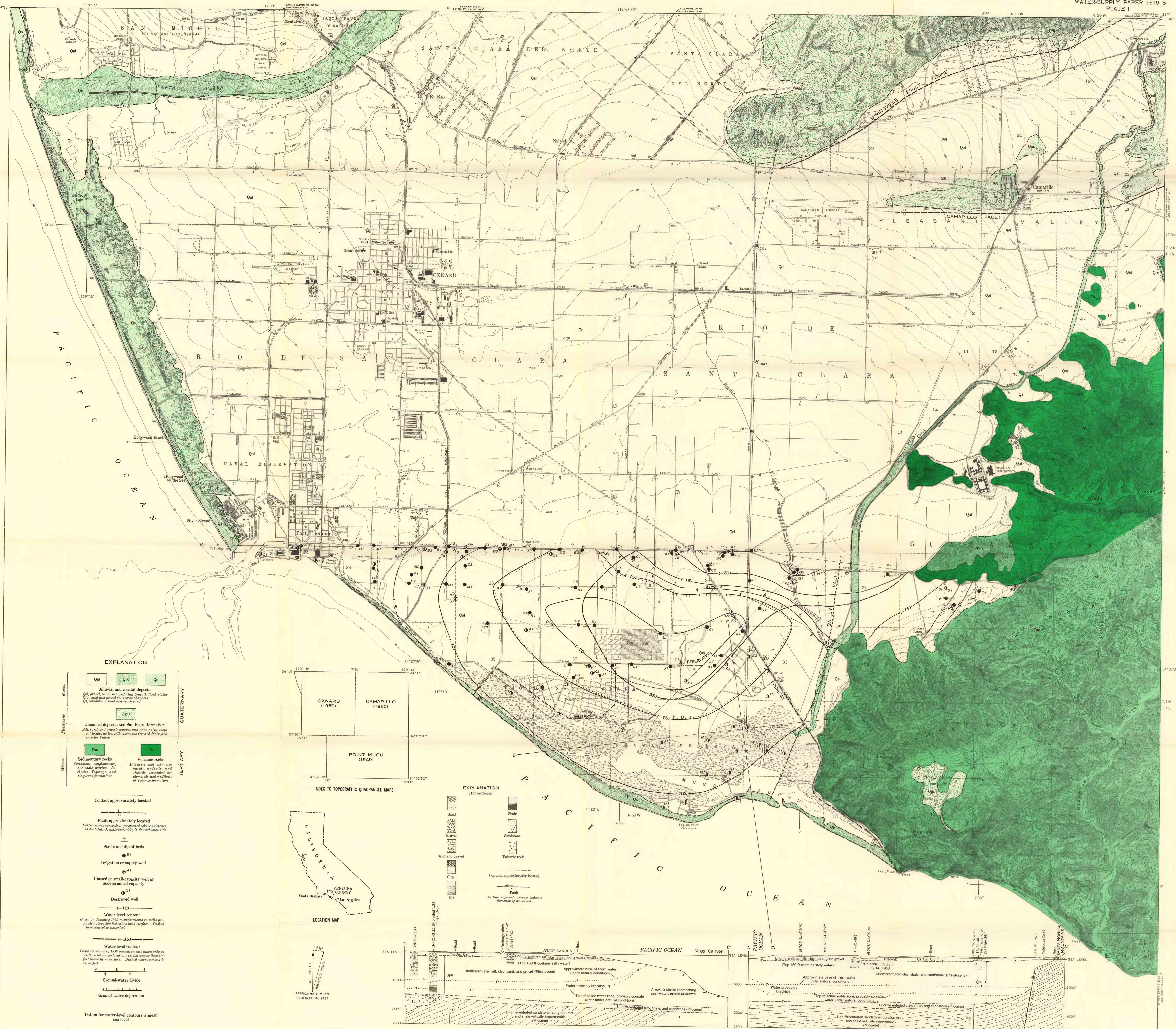
MAP AND SECTIONS OF THE NAVAL AIR MISSILE TEST CENTER AREA, POINT MUGU CALIFORNIA, SHOWING RECONNAISSANCE GEOLOGY, LOCATION OF WELLS, AND WATER-LEVEL CONTOURS IN JANUARY 1959
