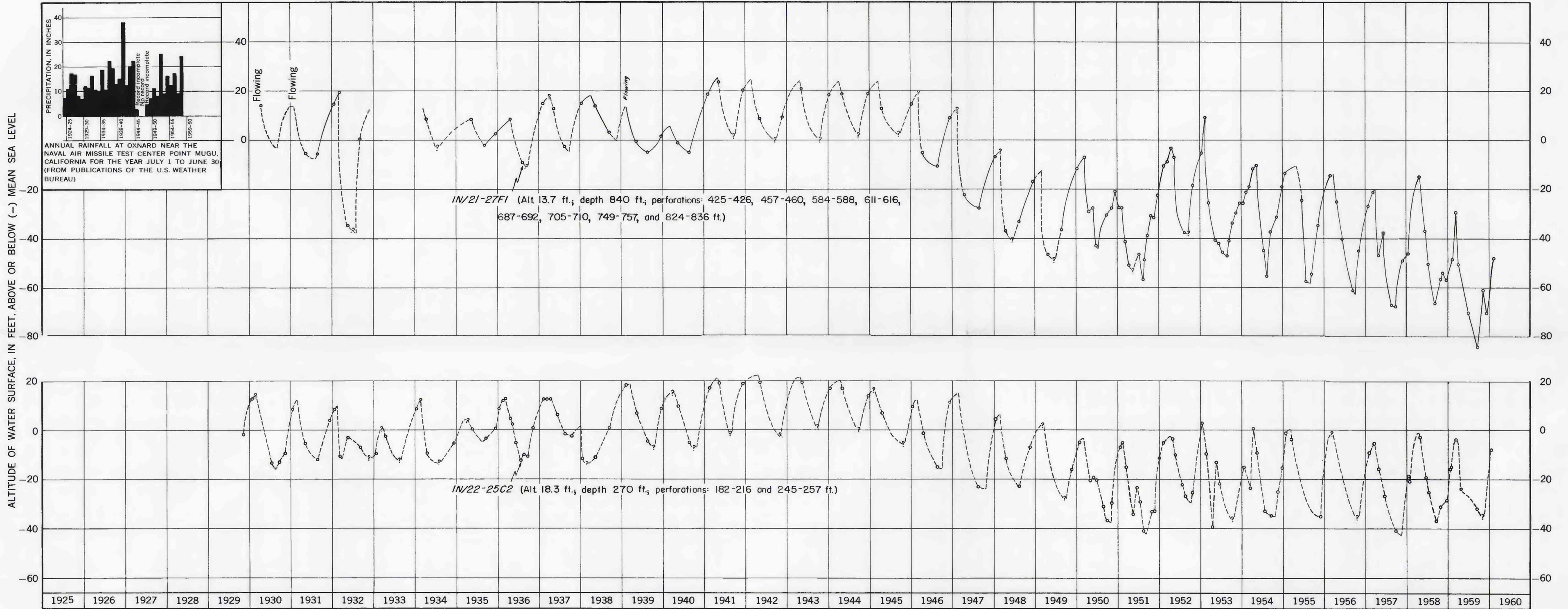
HYDROGRAPHS OF WELLS 1N/21-27F1 AND 1N/22-25C2
