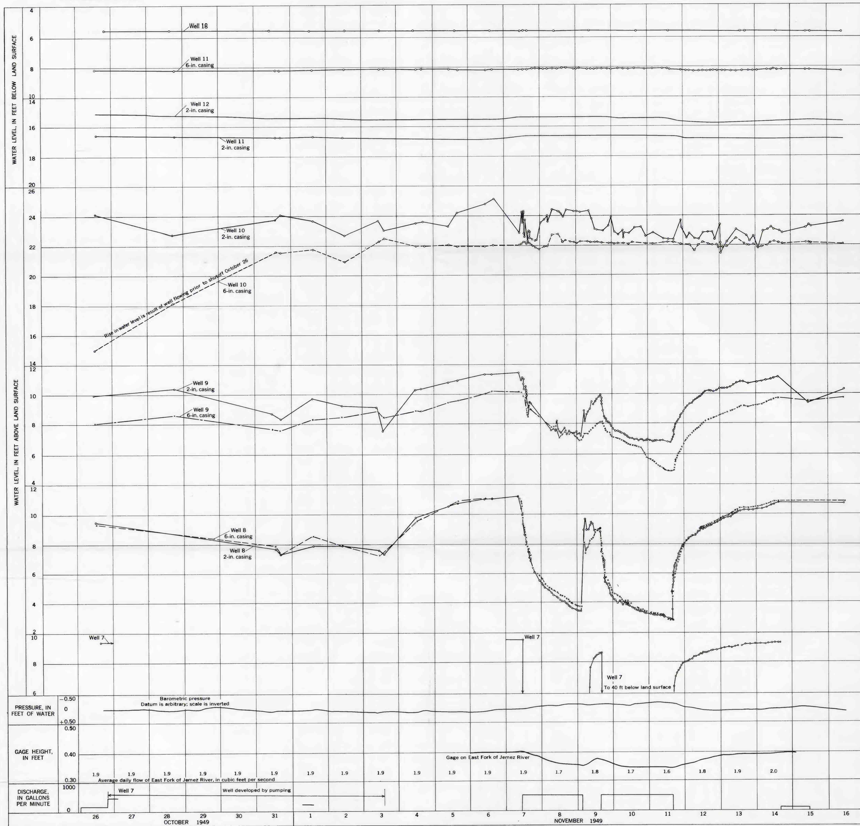
GRAPHIC PLOT OF THE WATER LEVEL IN WELLS 7-12 AND 18, THE RATE OF DISCHARGE OF WELL 7, AND THE BAROMETRIC PRESSURE FROM OCTOBER 26 TO NOVEMBER 16, 1949 IN THE VALLE GRANDE, SANDOVAL COUNTY, NEW MEXICO
