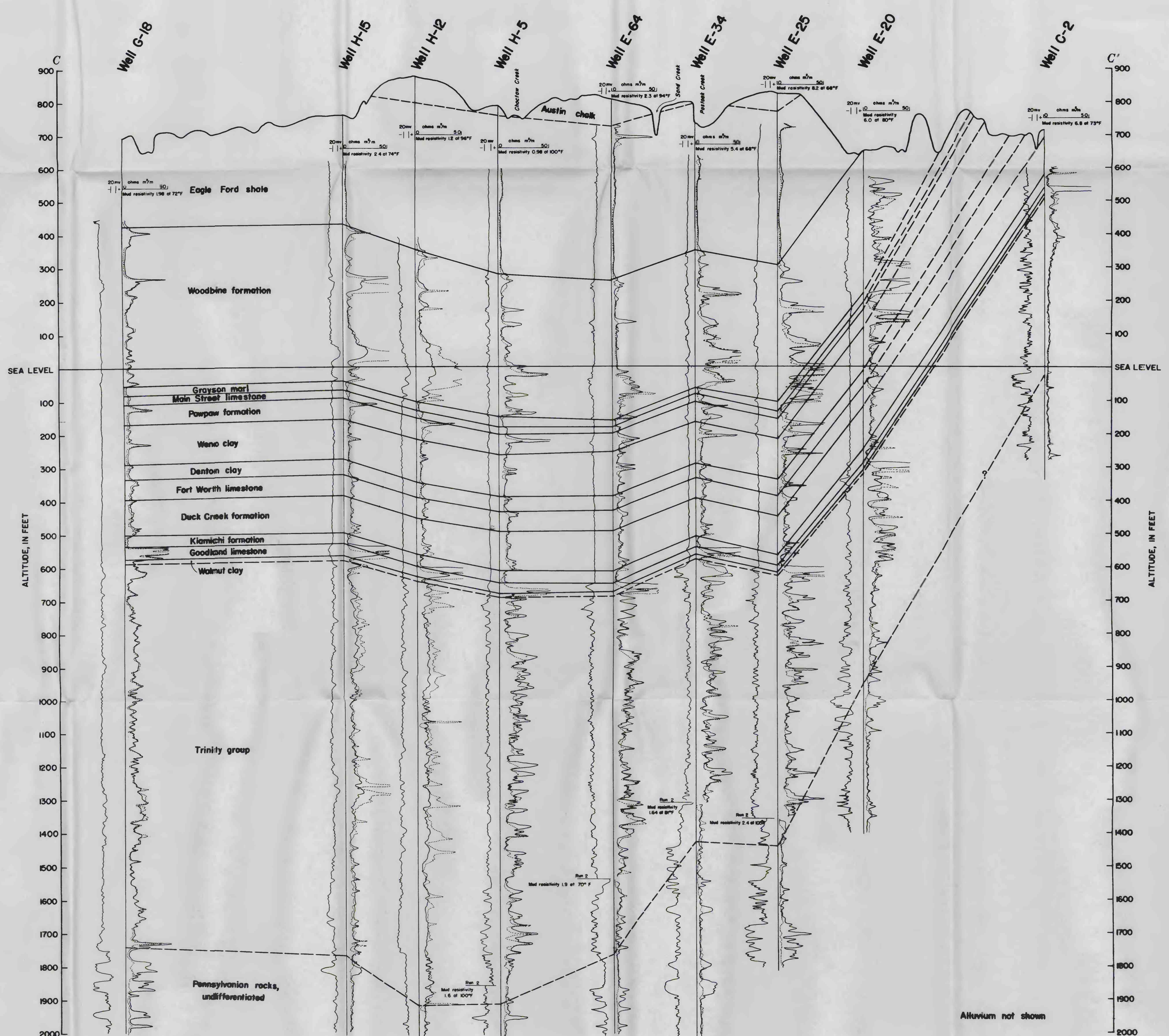
GEOLOGIC SECTIONS A-A', B-B', AND C-C' GRAYSON COUNTY, TEXAS
