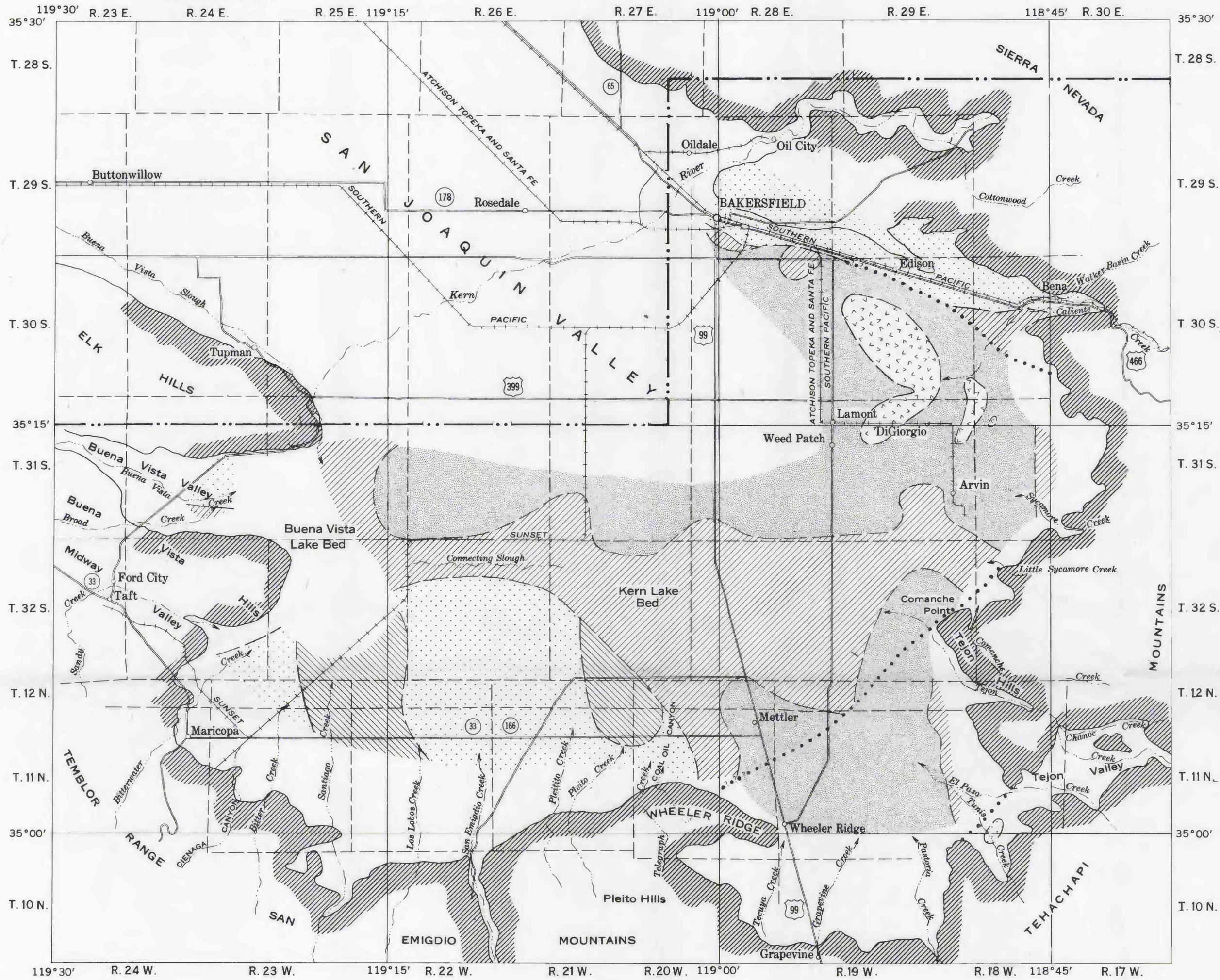
MAP SHOWING YIELD FACTORS OF SATURATED MATERIALS PENETRATED BY WELLS IN THE EDISON-MARICOPA AREA, CALIFORNIA
