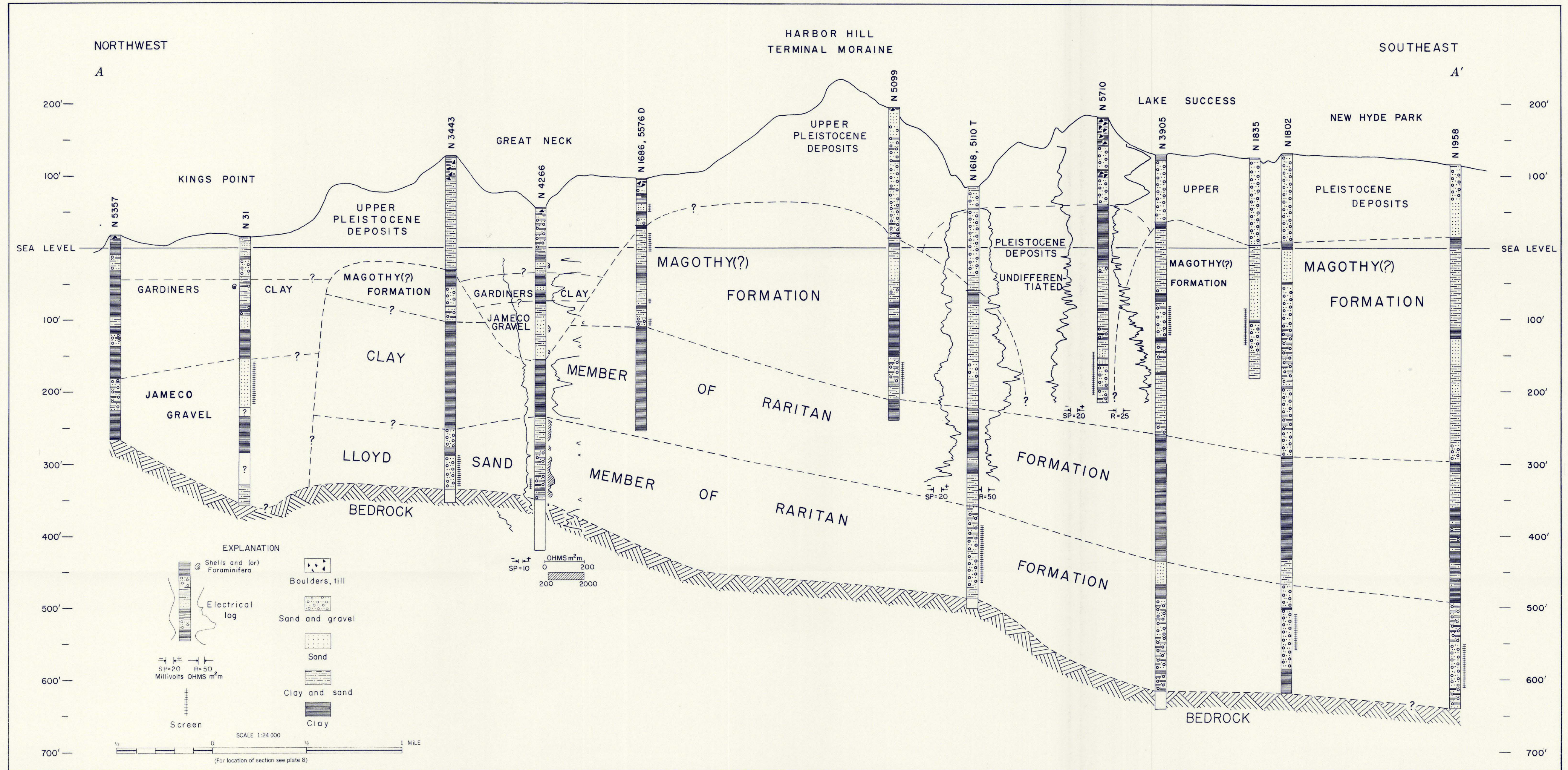
GEOLOGIC SECTION A-A' FROM KINGS POINT TO NEW HYDE PARK, NEW YORK
