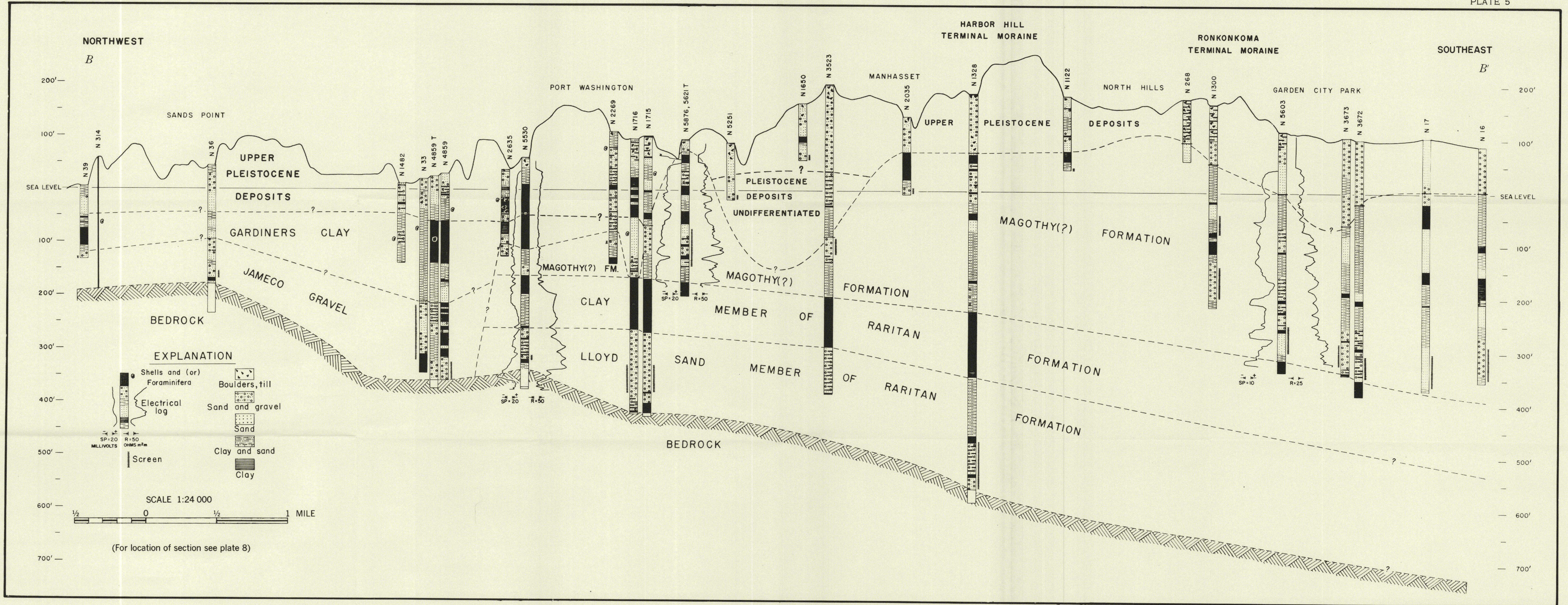
GEOLOGIC SECTION B-B' FROM SANDS POINT TO NEW HYDE PARK, NEW YORK
