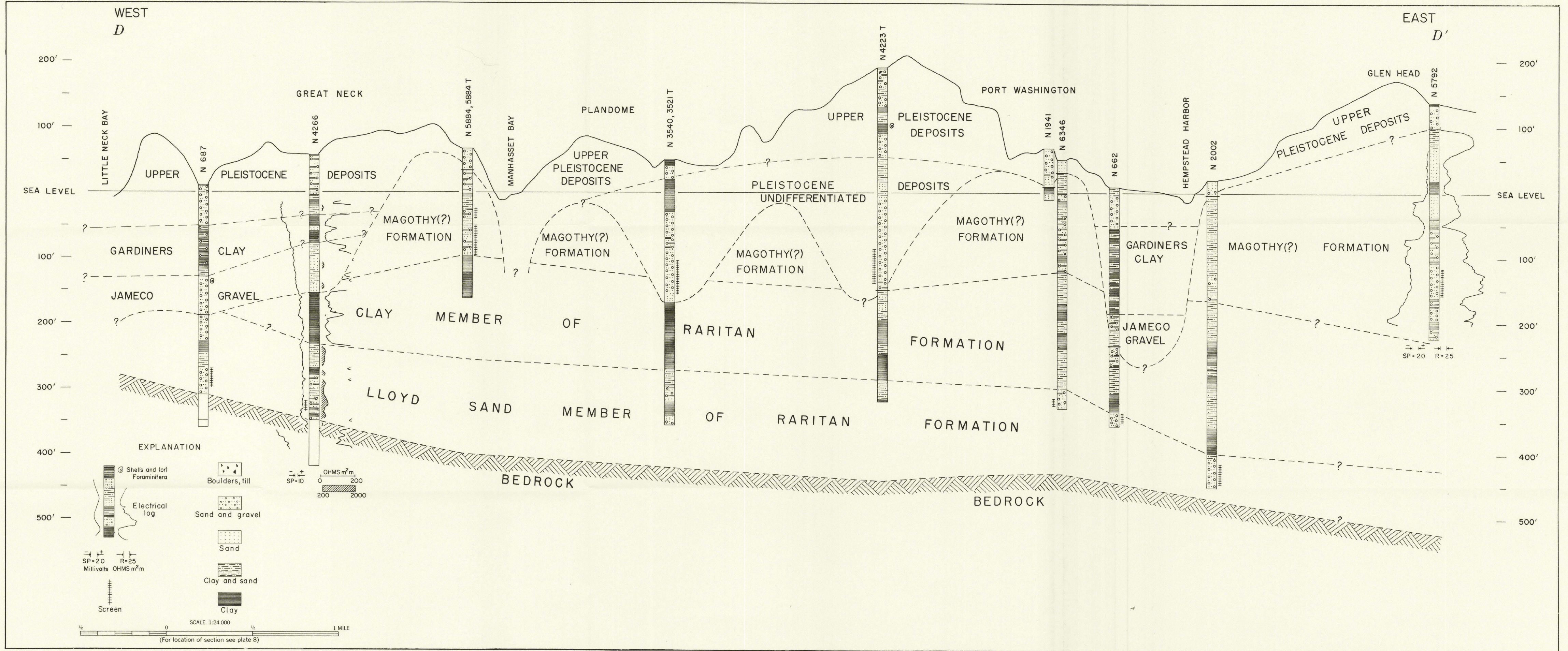
GEOLOGIC SECTION D-D' FROM GREAT NECK TO GLEN HEAD, NEW YORK
