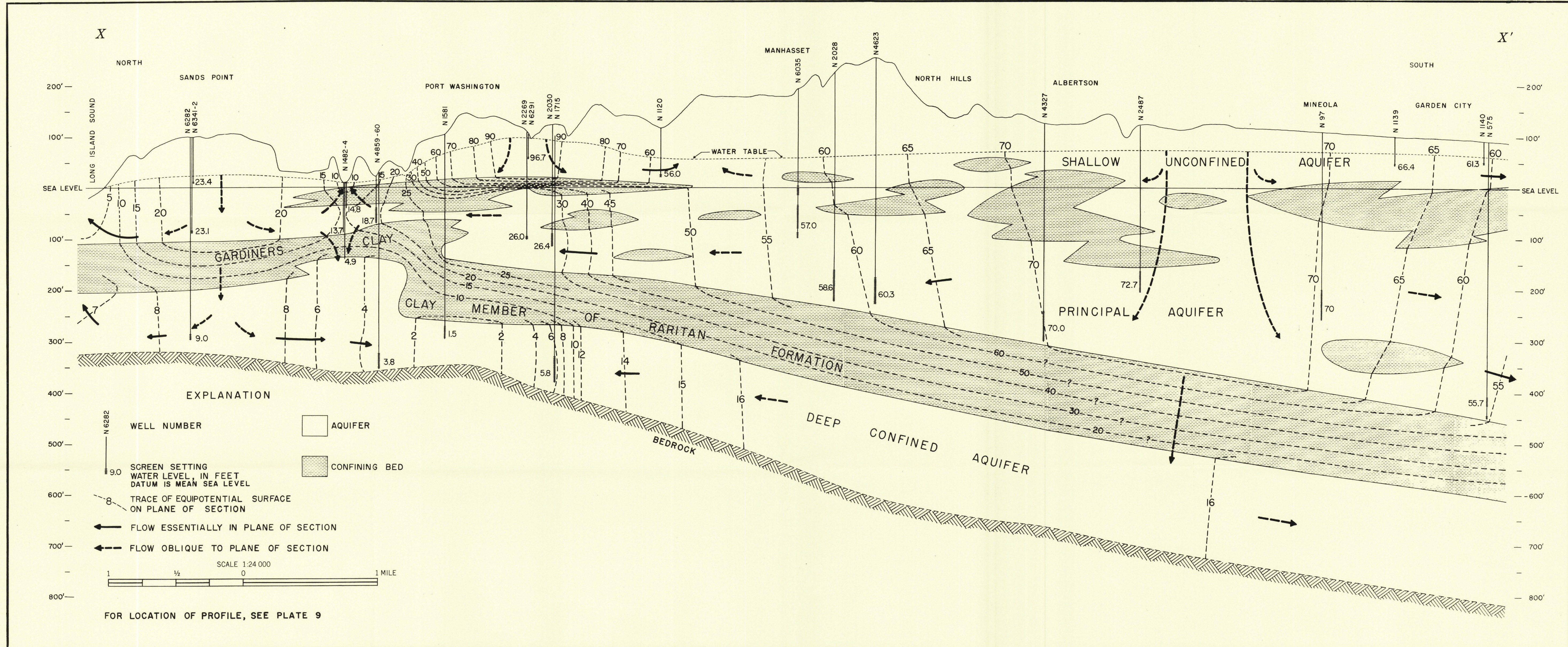
HYDRAULIC PROFILE THROUGH GROUND-WATER RESERVOIR ALONG LINE X-X' FROM SANDS POINT TO GARDEN CITY, NEW YORK, APRIL 1957
