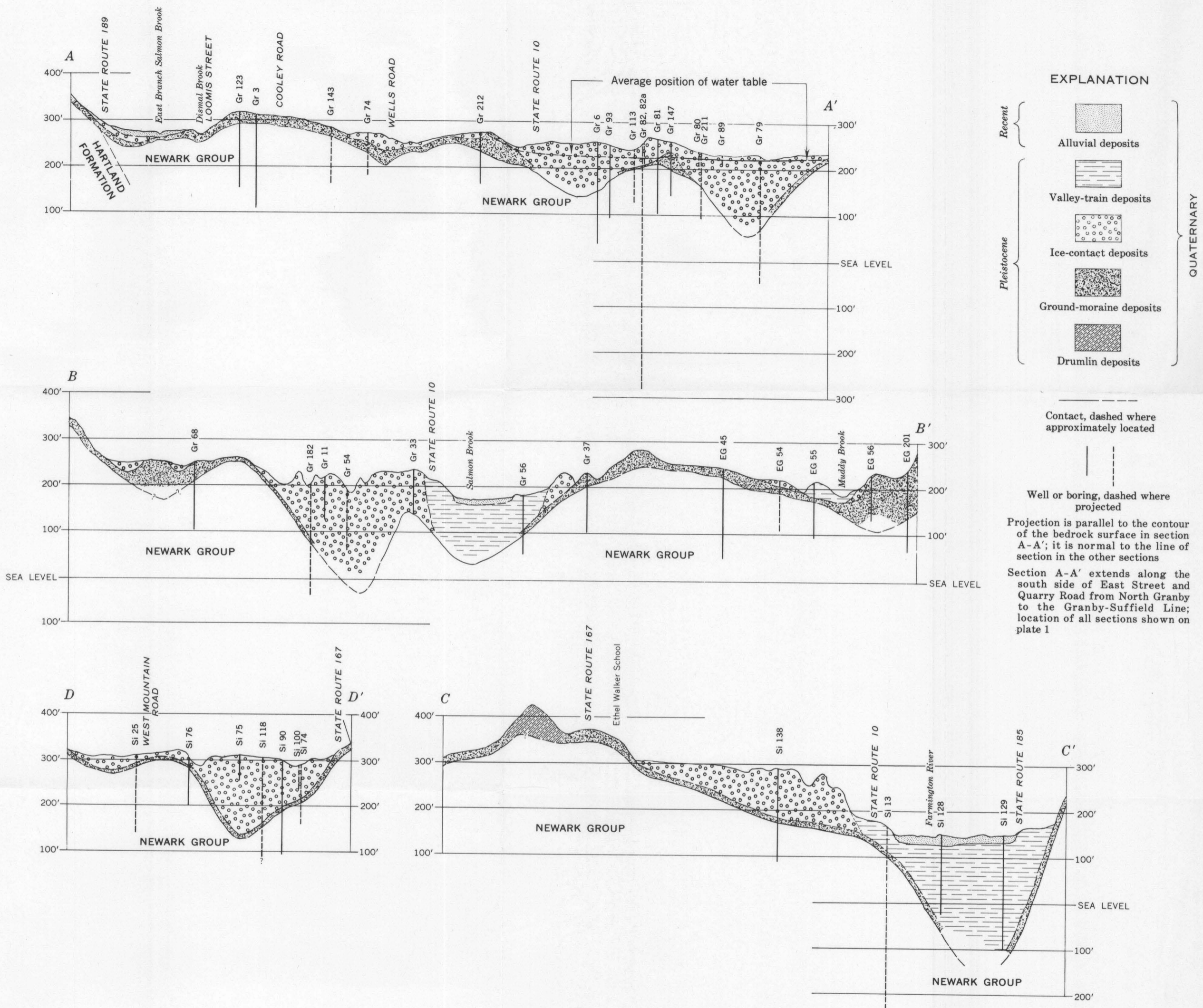
GEOLOGIC SECTIONS OF THE FARMINGTON-GRANBY AREA, CONNECTICUT
