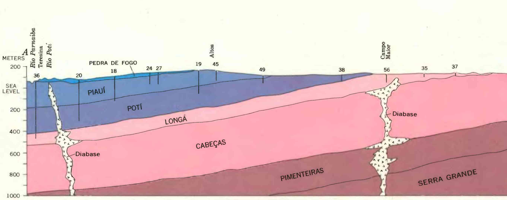
A. GENERALIZED GEOLOGY
