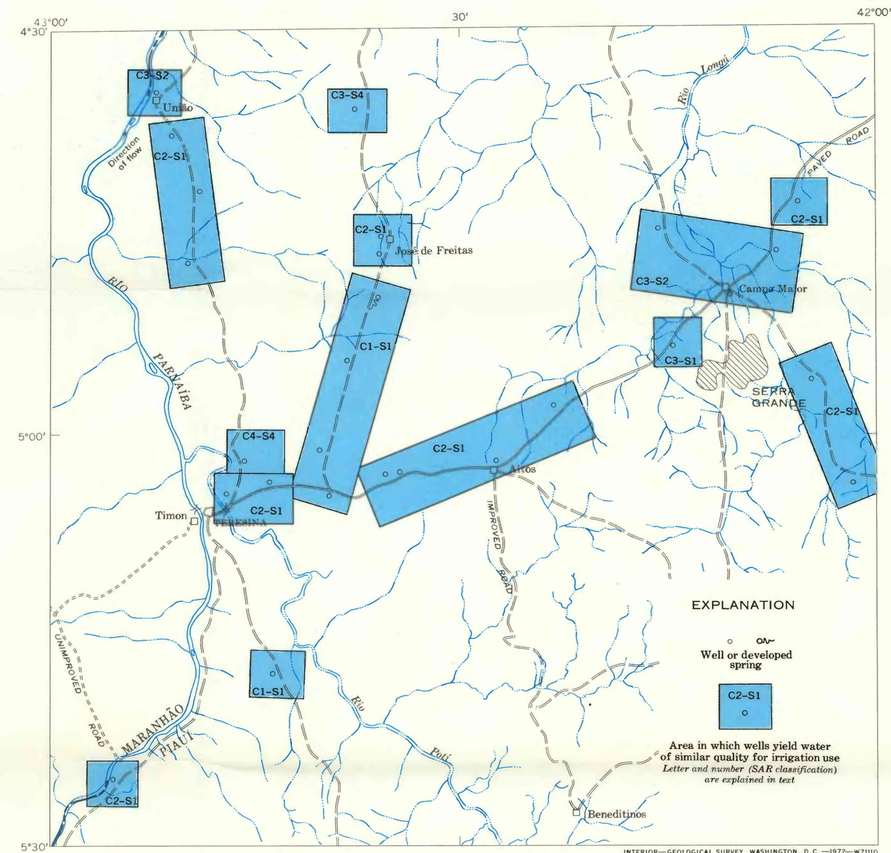
D. CLASSIFICATION OF GROUND WATER FOR IRRIGATION USE
