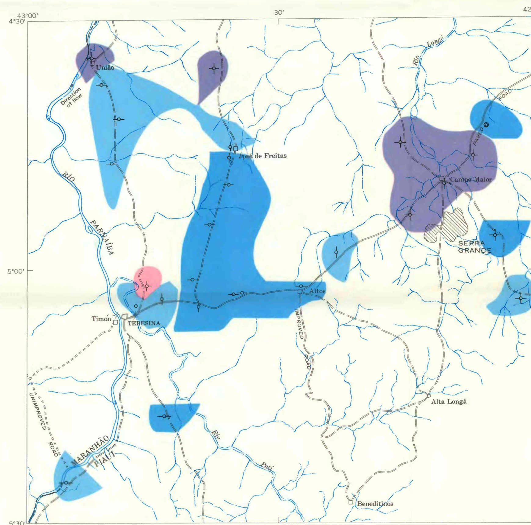
C. GEOGRAPHIC AND GEOLOGIC DISTRIBUTION OF DISSOLVED SOLIDS IN WATER FROM PRINCIPAL AQUIFERS
