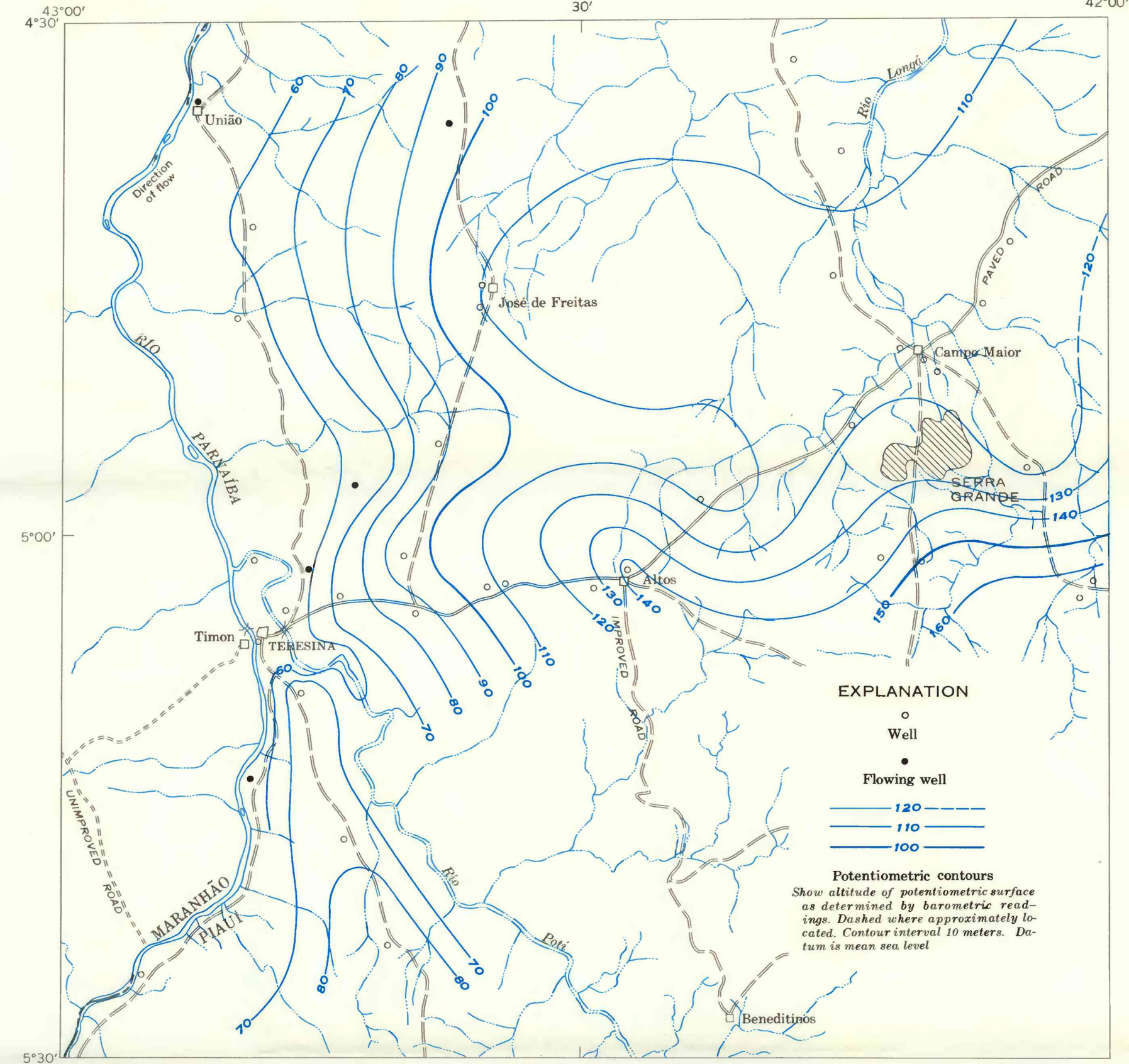
B. CONFIGURATION OF POTENTIOMETRIC SURFACE
