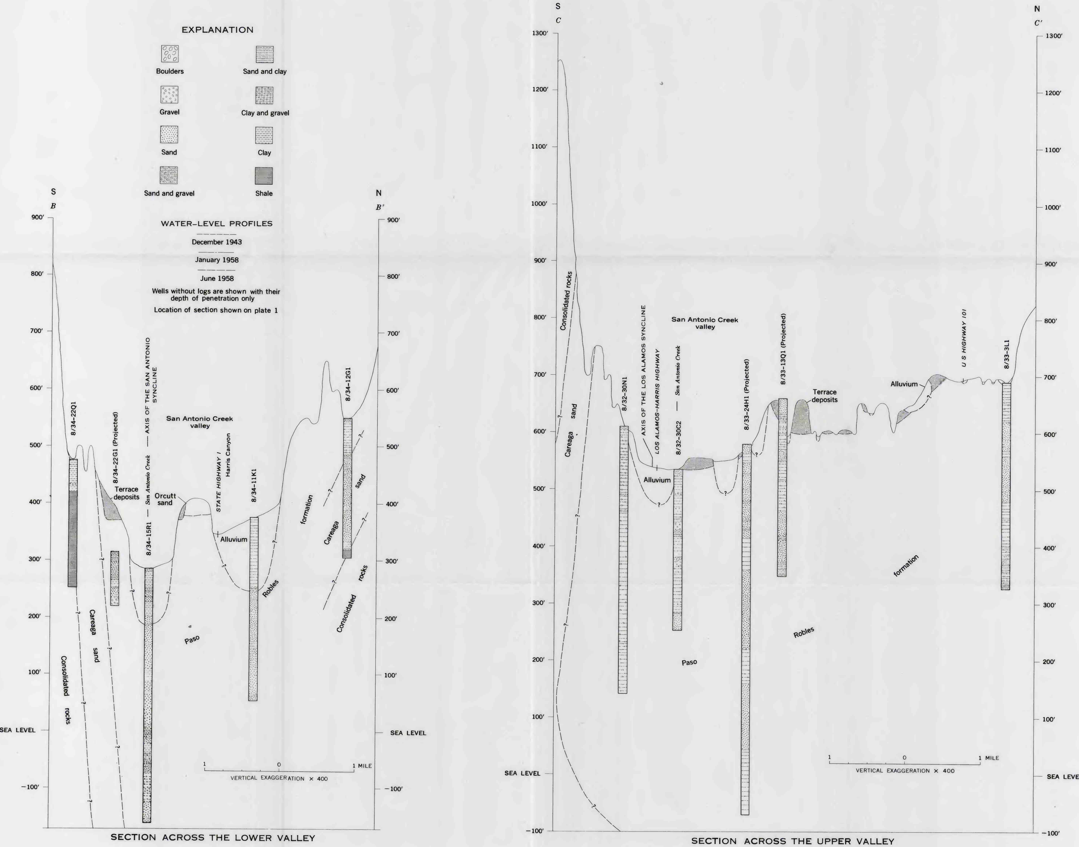
GEOLOGIC STRUCTURE ALONG THE SAN ANTONIO CREEK VALLEY, CALIFORNIA
