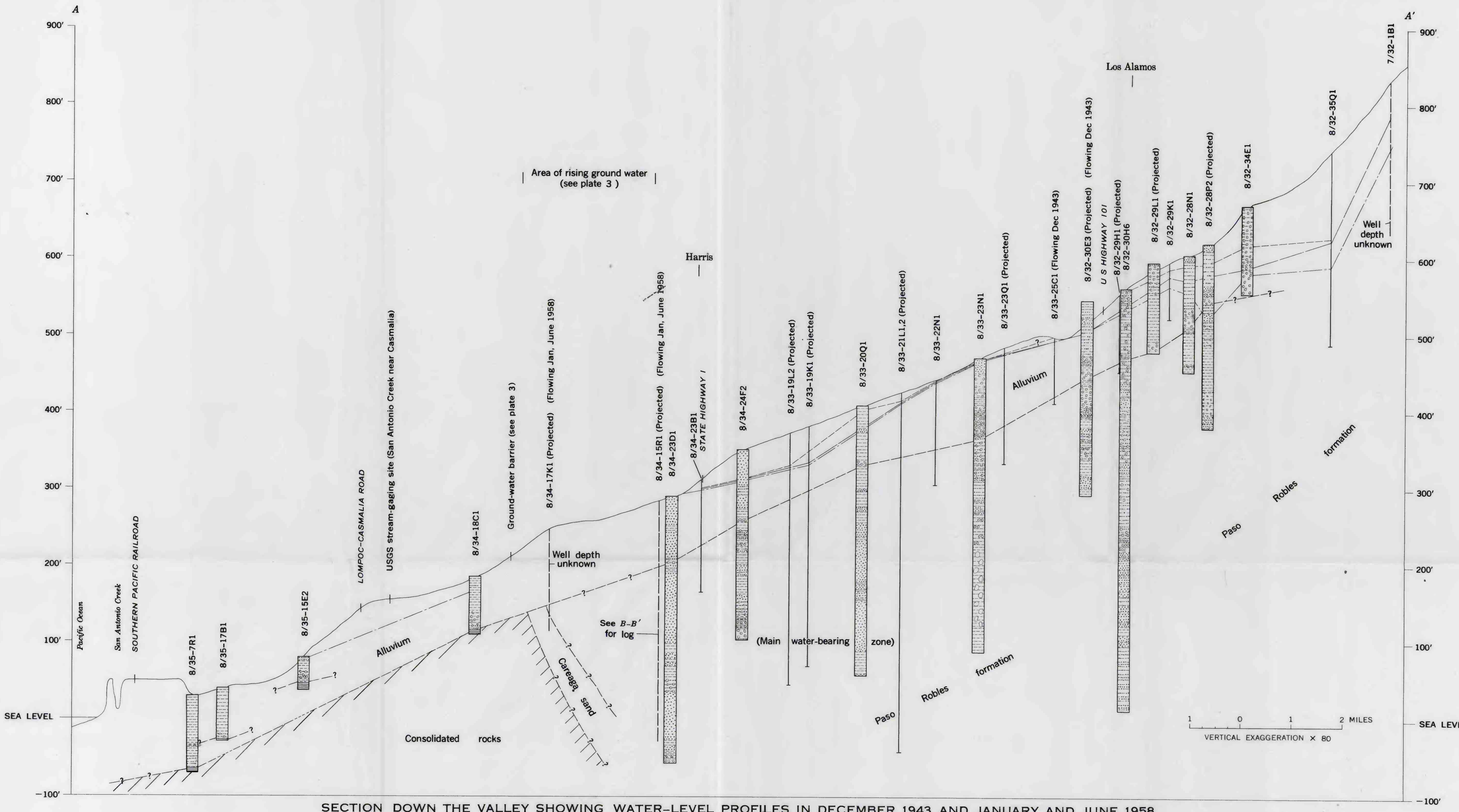
SECTION DOWN THE VALLEY SHOWING WATER-LEVEL PROFILES IN DECEMBER 1943 AND JANUARY AND JUNE 1958
