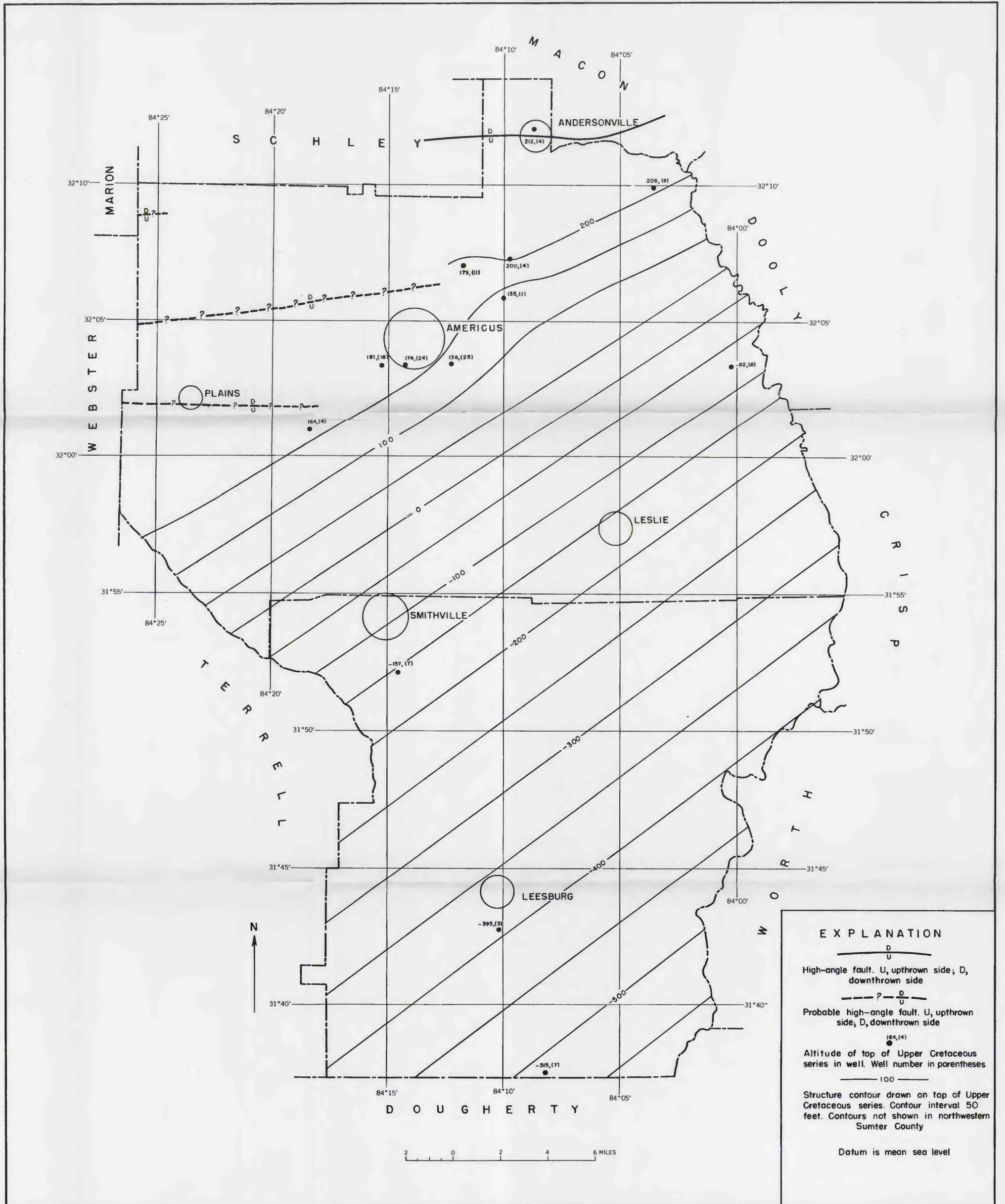
MAP SHOWING STRUCTURAL CONTOURS ON THE TOP OF UPPER CRETACEOUS SERIES, LEE AND SUMTER COUNTIES, GEORGIA
