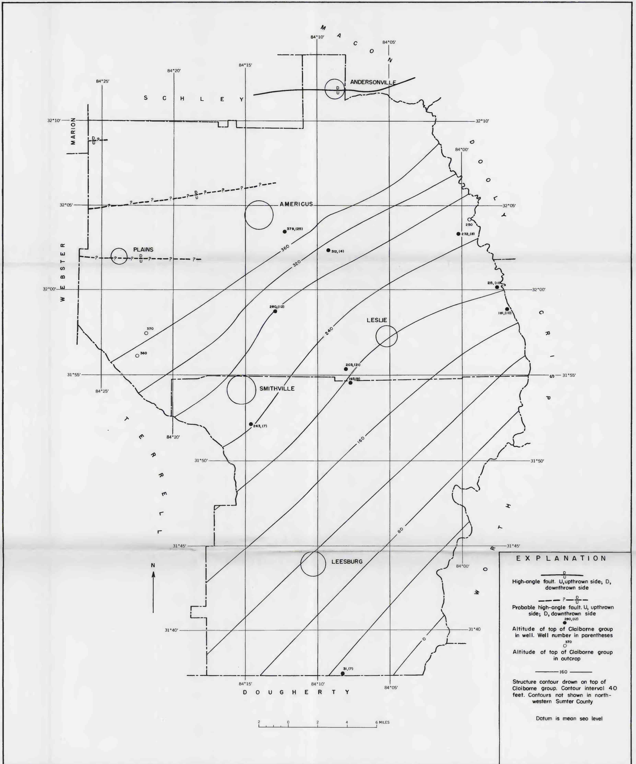
MAP SHOWING STRUCTURAL CONTOURS ON THE TOP OF CLAIBORNE GROUP
