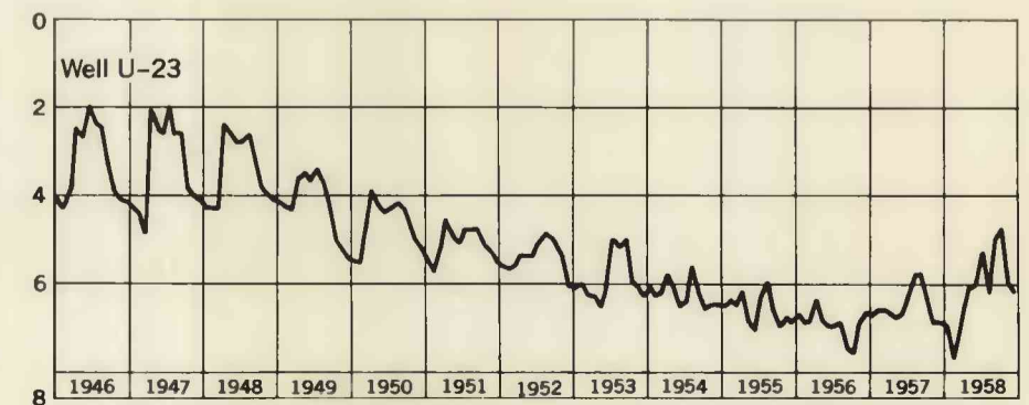
FLUCTUATIONS OF WATER LEVELS IN SHALLOW WELLS IN THE LOWER MESILLA VALLEY, 1946-58
