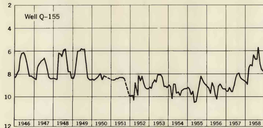
FLUCTUATIONS OF WATER LEVELS IN SHALLOW WELLS IN THE LOWER MESILLA VALLEY, 1946-58
