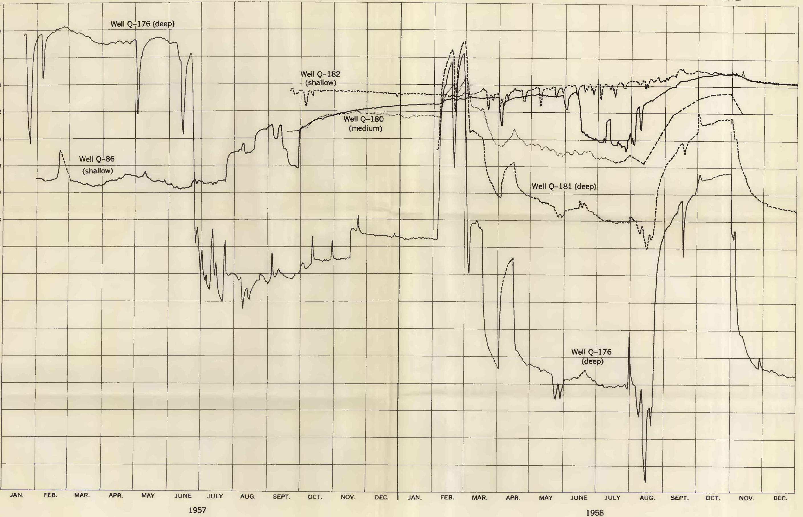
FLUCTUATIONS OF WATER LEVELS IN WELLS IN THE EL PASO CITY WELL FIELD, TEXAS, NORTHWEST OF CANUTILLO, 1957-58
