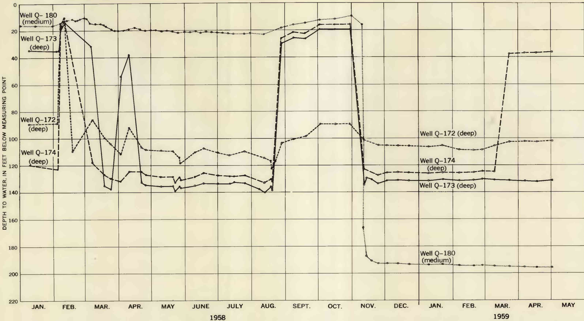
FLUCTUATIONS OF WATER LEVELS IN WELLS IN THE EL PASO CITY WELL FIELD, TEXAS, NORTHWEST OF CANUTILLO, 1958-59
