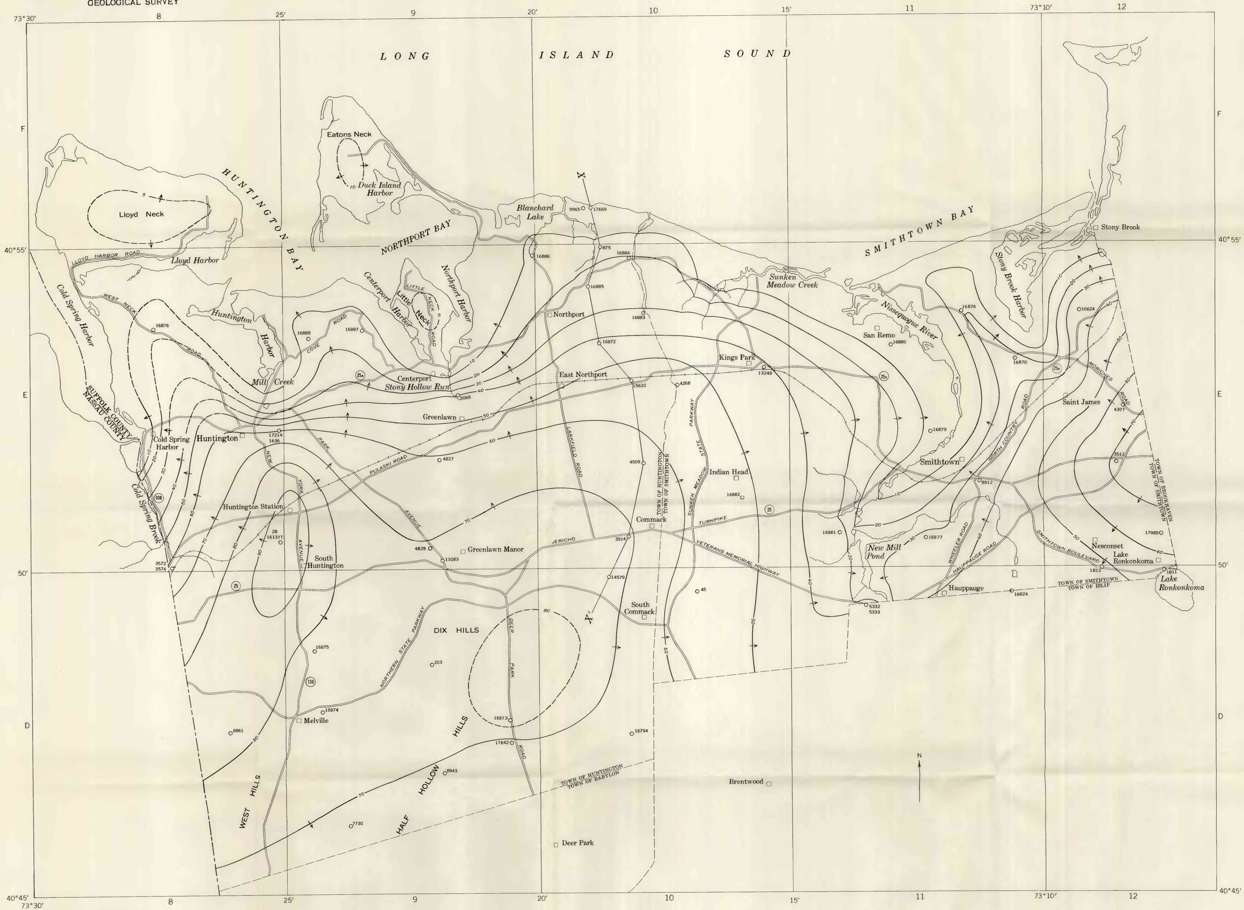
MAP OF THE HUNTINGTON-SMITHTOWN AREA, SUFFOLK COUNTY, NEW YORK, SHOWING CONTOURS ON THE WATER TABLE OF THE SHALLOW AQUIFER IN MAY, 1959
