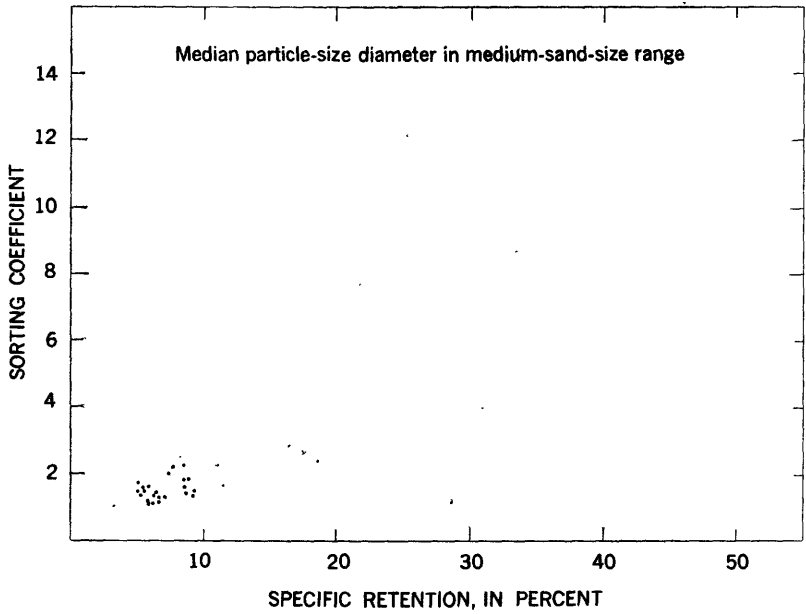
FIGURE 7.—Relation between sorting-coefficient and specific-retention values of samples from the Humboldt River valley, fine- and medium- sand-size ranges.
