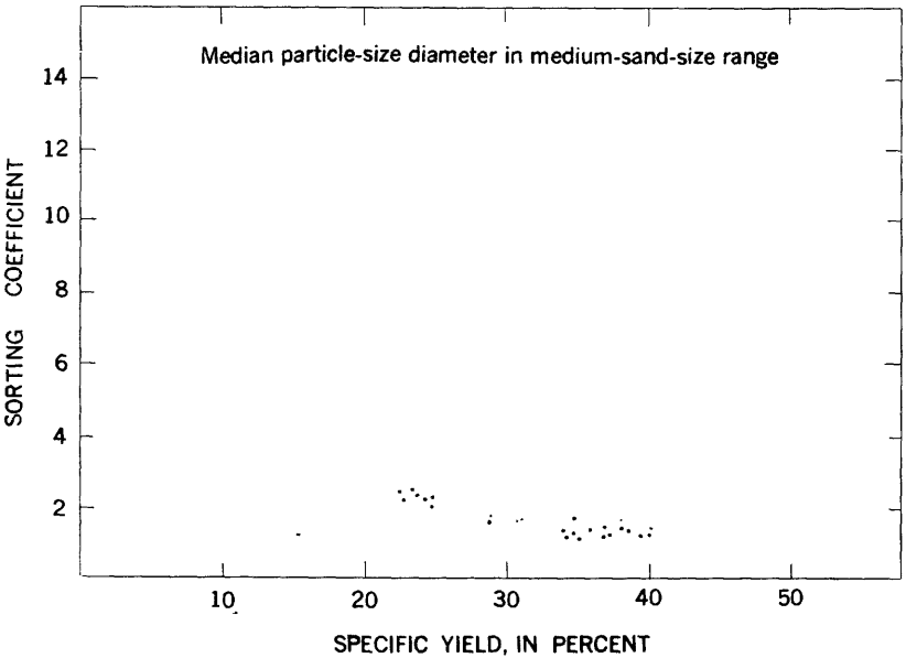
FIGURE 12.—Relation between sorting-coefficient and specific-yield values of samples from the Humboldt River valley, fine- and medium-sand-size ranges.
