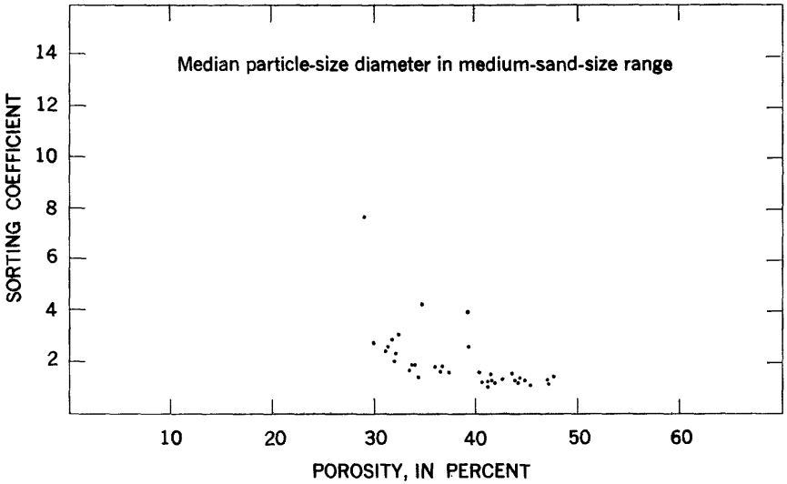
FIGURE 3.—Relation between porosity and sorting-coefficient values of samples from the Humboldt River valley, fine- and medium-sand-size ranges.
