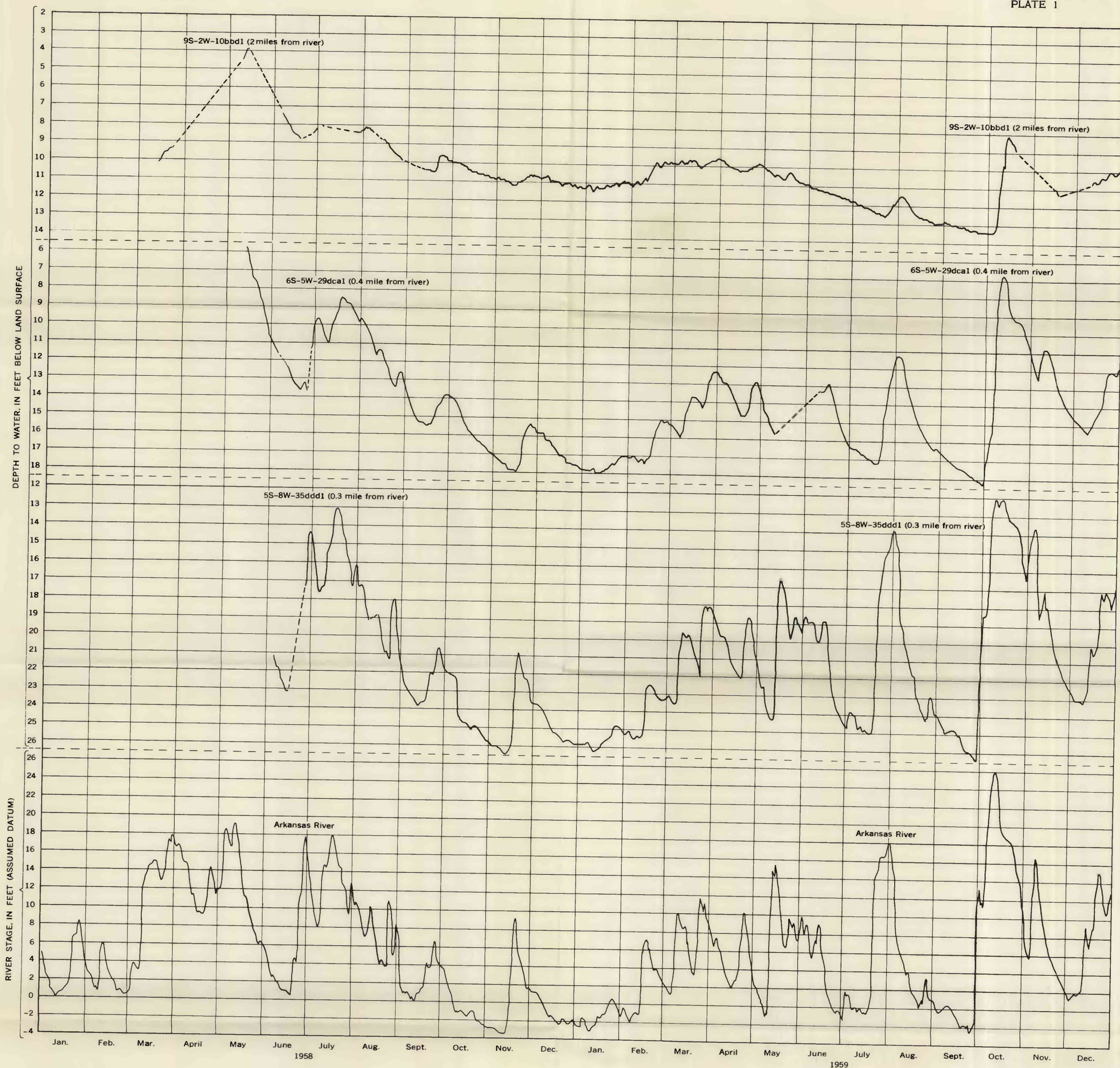
HYDROGRAPHS OF THE ARKANSAS RIVER AT THE U.S. WEATHER BUREAU GAGE AT PINE BLUFF, ARKANSAS AND WELLS 9S-2W-10bdd1, 6S-5W-29dca1, AND 5S-8W-35ddd1
