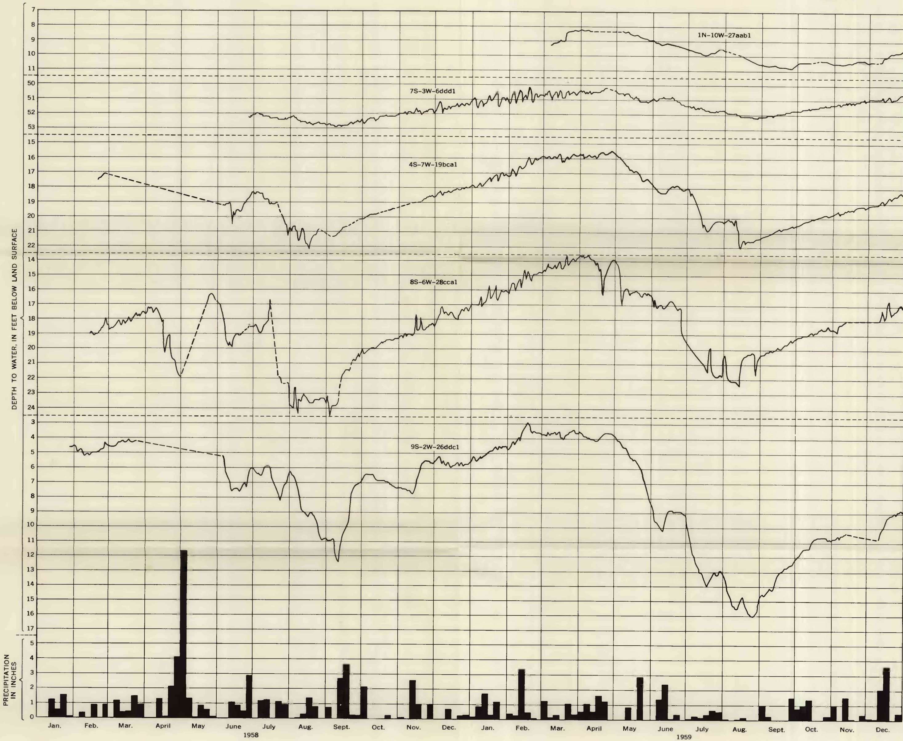
HYDROGRAPHS OF WELLS 1N-10W-27aab1, 7S-3W-6ddd1, 4S-7W-19bca1, 8S-6W-28cca1, AND 9S-2W-26ddc1 AND PRECIPITATION AT PINE BLUFF, ARKANSAS
