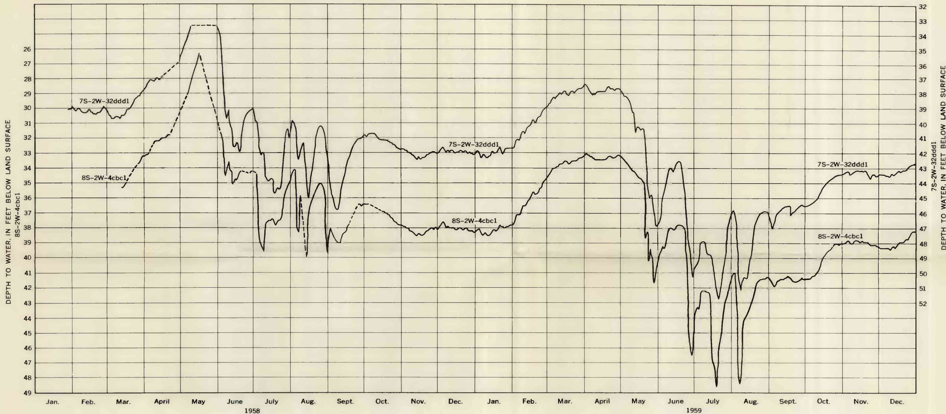
HYDROGRAPHS OF WELLS 7S-2W-32ddd1 AND 8S-2W-4cbc1, ARKANSAS RIVER VALLEY, ARKANSAS
