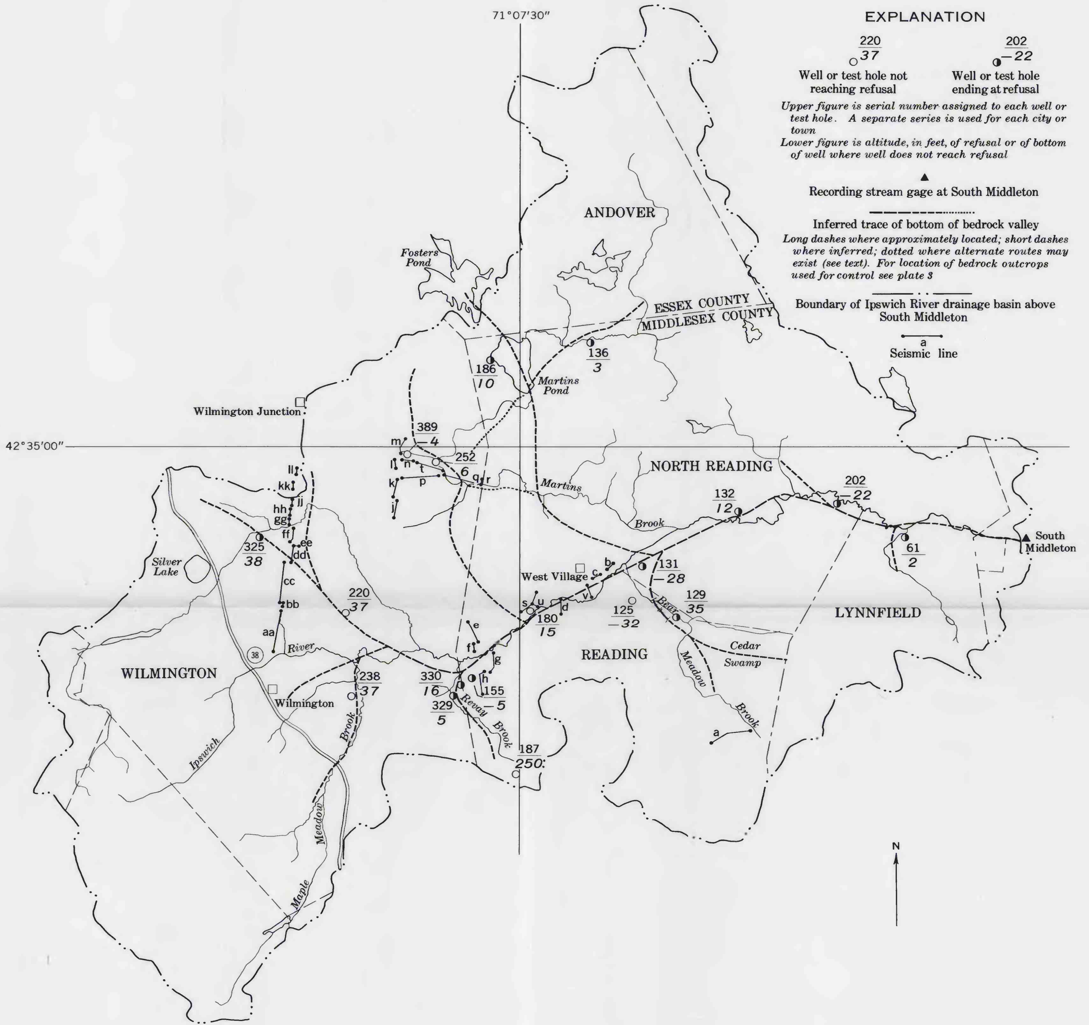
MAP OF THE WILMINGTON-READING AREA, MASSACHUSETTS, SHOWING INFERRED TRACES OF BURIED VALLEYS
