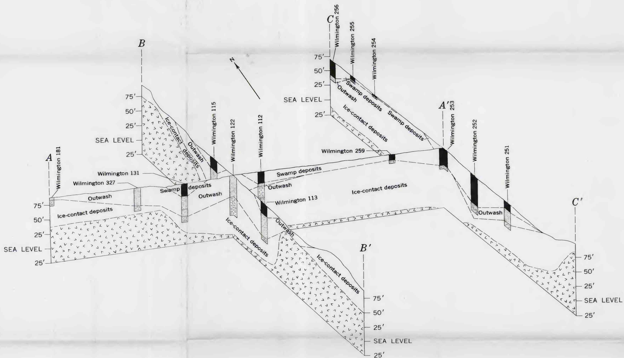
FENCE DIAGRAM OF THE SALEM STREET WELL FIELD, WILMINGTON, MASSACHUSETTS
