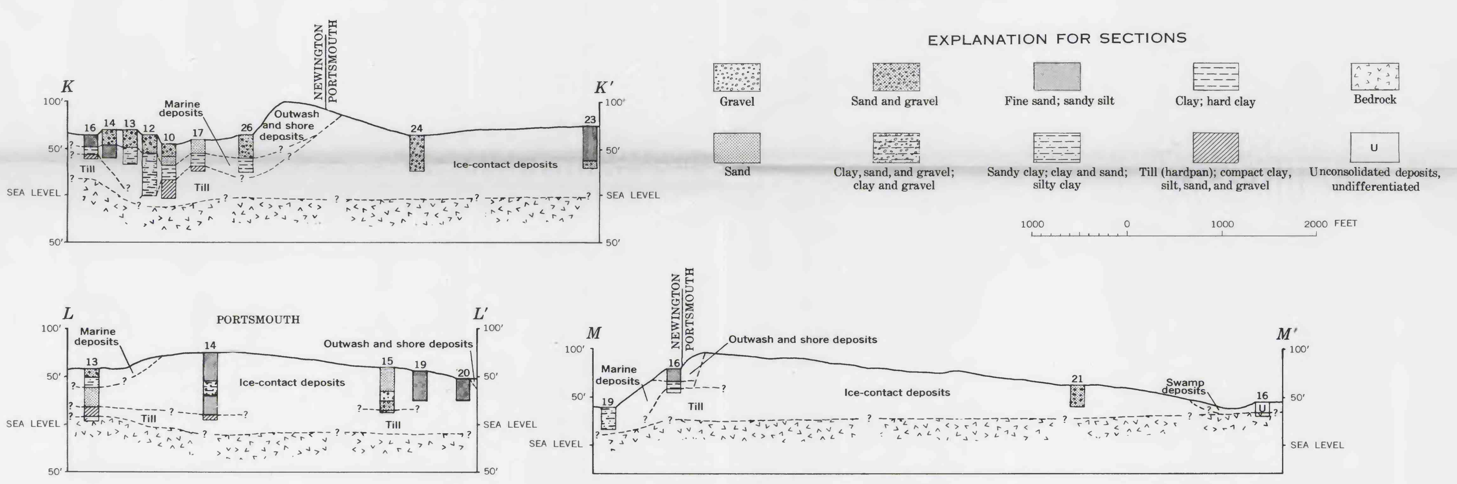
GEOLOGIC MAP AND SECTIONS OF AREA D SHOWING UNCONSOLIDATED DEPOSITS AND LOCATION OF SELECTED WELLS, TEST HOLES, AND SPRINGS
