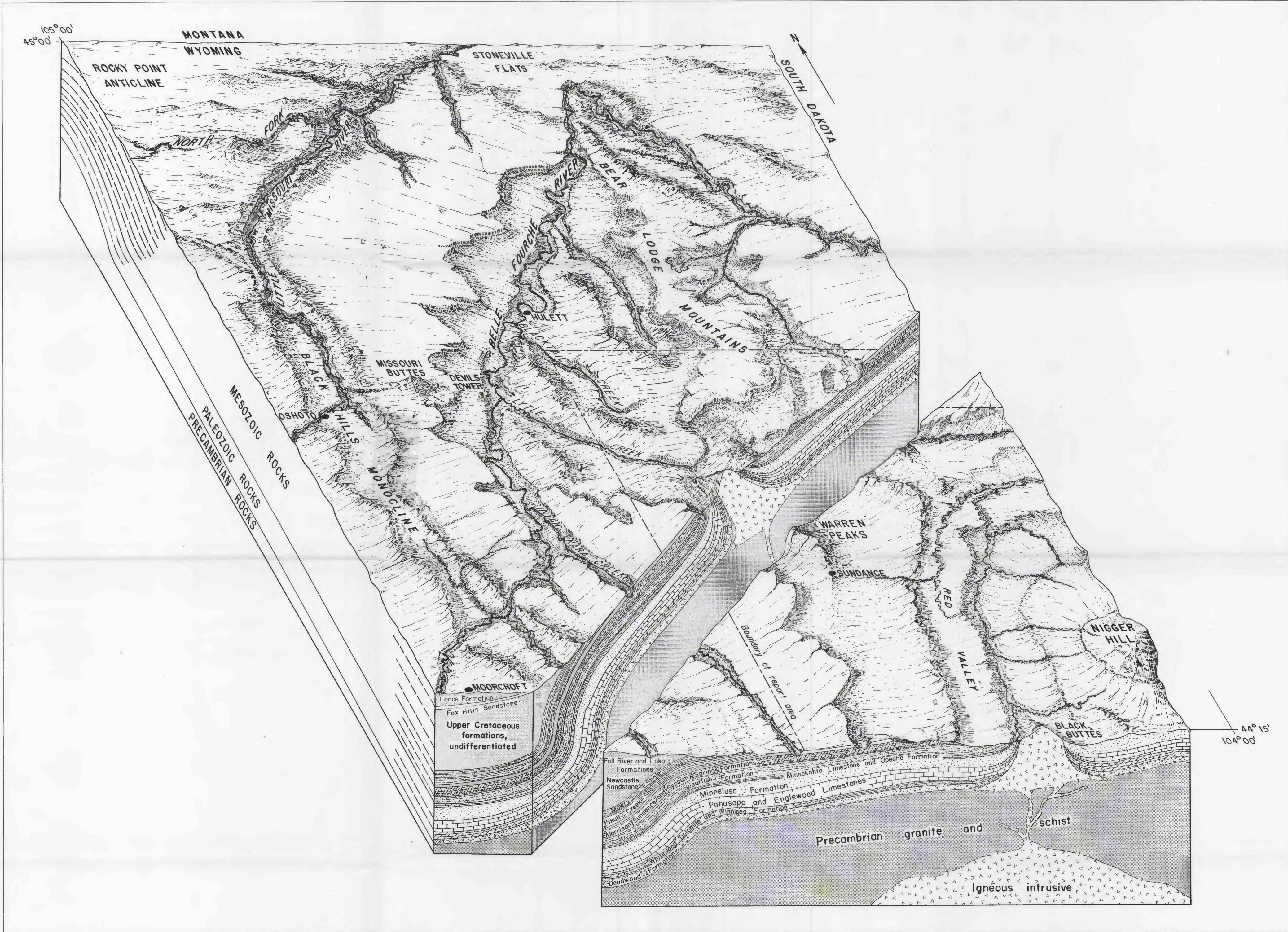
BLOCK DIAGRAM OF A PART OF CROOK COUNTY, WYOMING, SHOWING THE PHYSIOGRAPHY, GENERAL STRUCTURE, AND OUTLINE OF THE REPORT AREA
