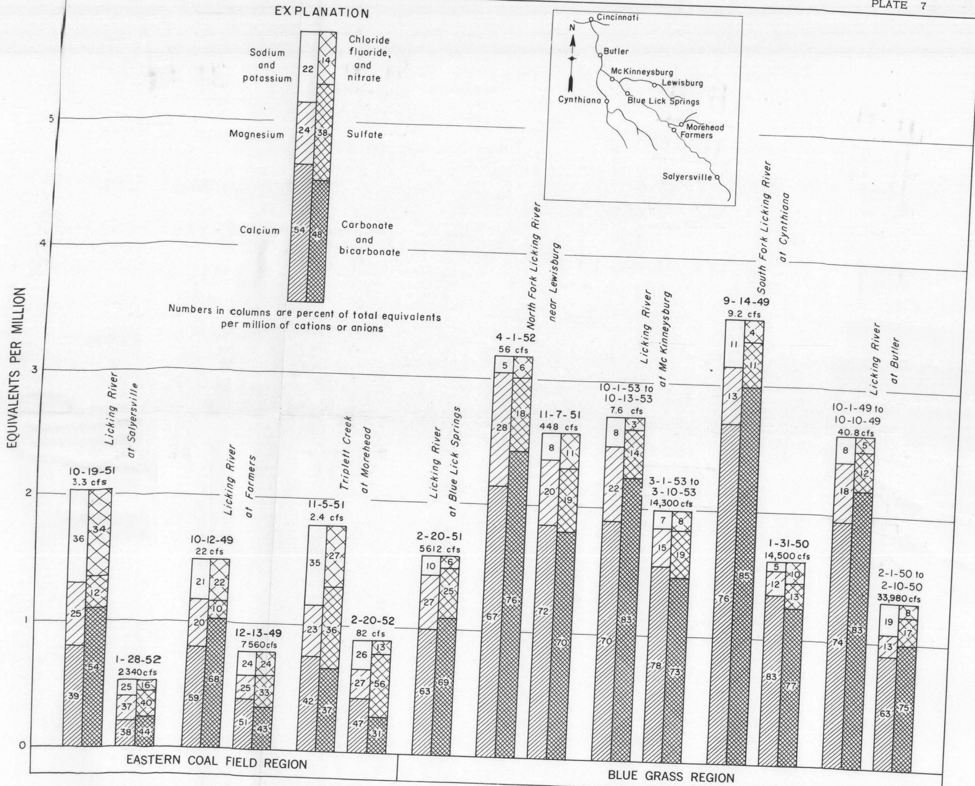
CHEMICAL CHARACTERISTICS OF SURFACE WATER IN THE LICKING RIVER BASIN, KENTUCKY AT LOW AND HIGH RATES OF DISCHARGE
