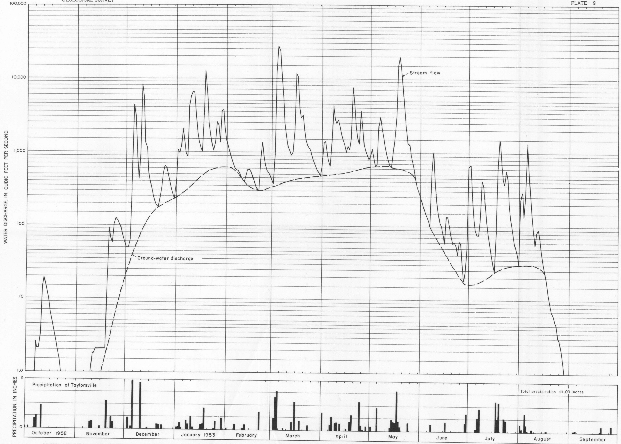
RELATION OF MEAN DAILY RUNOFF TO GROUND-WATER DISCHARGE, SALT RIVER AT SHEPHERDSVILLE, OCTOBER 1, 1952 TO SEPTEMBER 30, 1953
