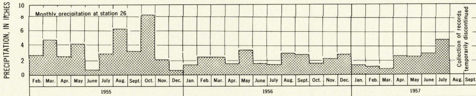
GRAPHS SHOWING THE DAILY HIGHEST AND LOWEST WATER LEVELS IN WELL Sa 843, THE STAGE OF KAYADEROSSERAS CREEK, AND MONTHLY PRECIPITATION AT STATION 26
