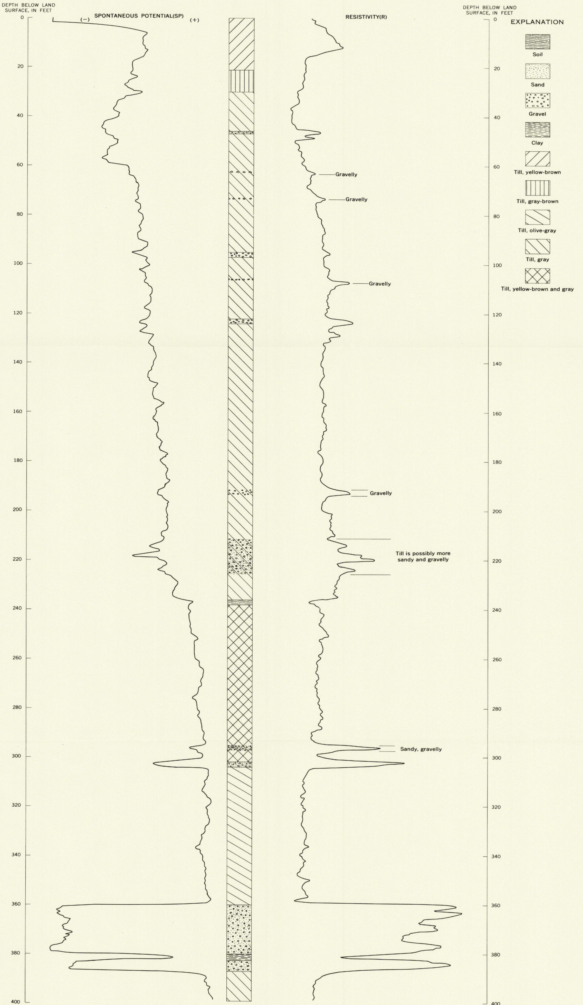
ELECTRIC AND SAMPLE LOGS OF TEST HOLE 101.41.22bab1, NOBLES COUNTY, MINNESOTA, SHOWING CHARACTERISTIC ELECTRICAL RESPONSES IN GLACIAL DRIFT
