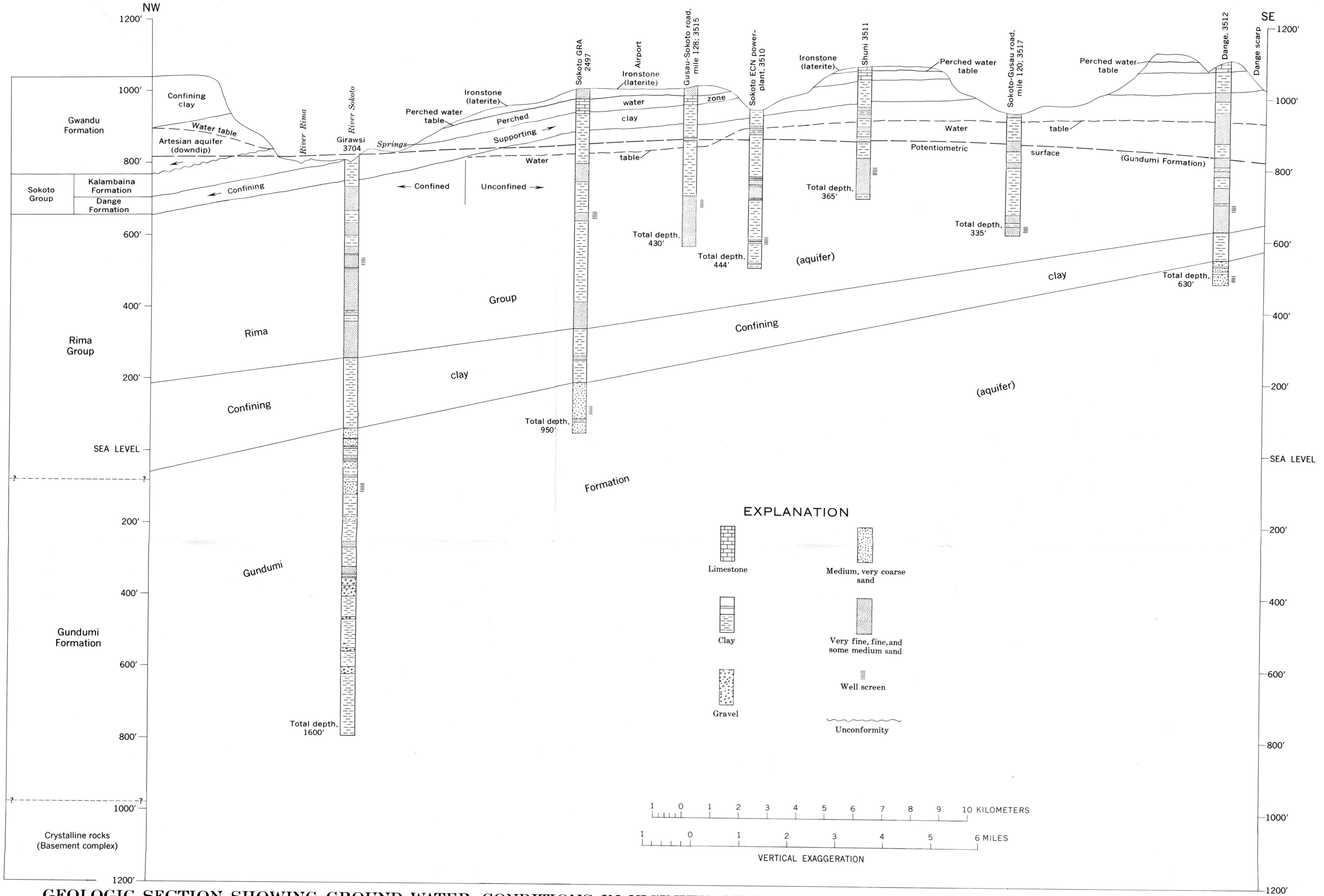
GEOLOGIC SECTION SHOWING GROUND-WATER CONDITIONS IN VICINITY OF SOKOTO, SOKOTO BASIN, NORTHWESTERN NIGERIA
