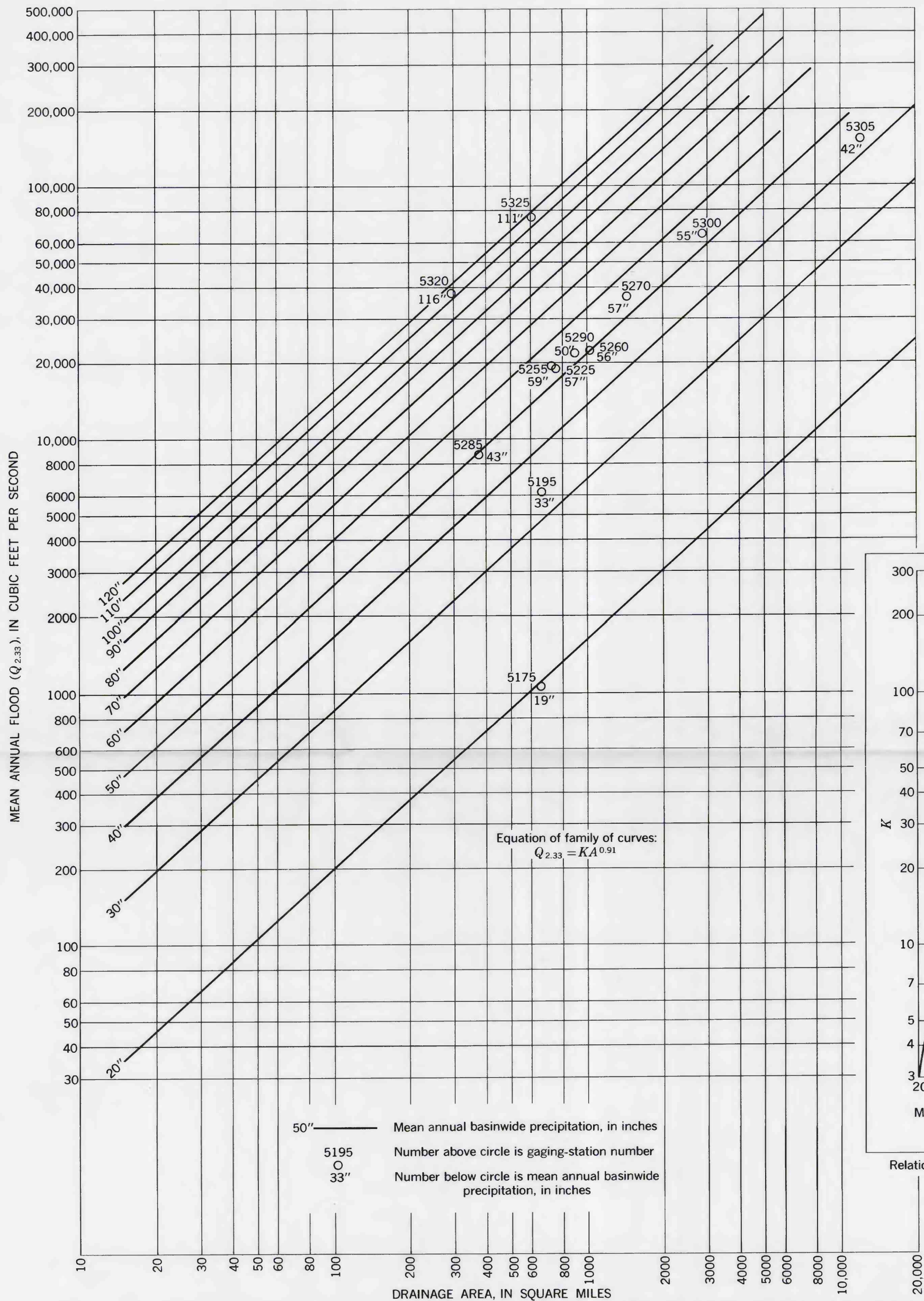
RELATION OF MEAN ANNUAL FLOOD, DRAINAGE AREA, AND MEAN ANNUAL BASINWIDE PRECIPITATION IN THE KLAMATH MOUNTAINS
