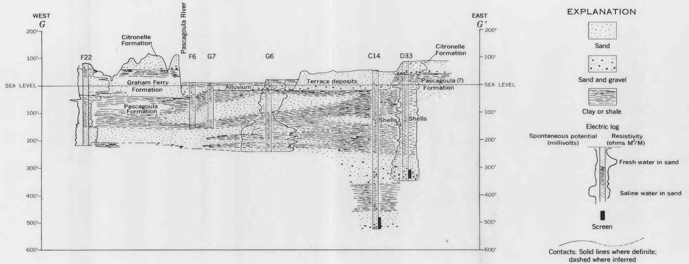
GEOLOGIC SECTION G-G' ACROSS PASCAGOULA RIVER AT GRAHAM FERRY, MISSISSIPPI
