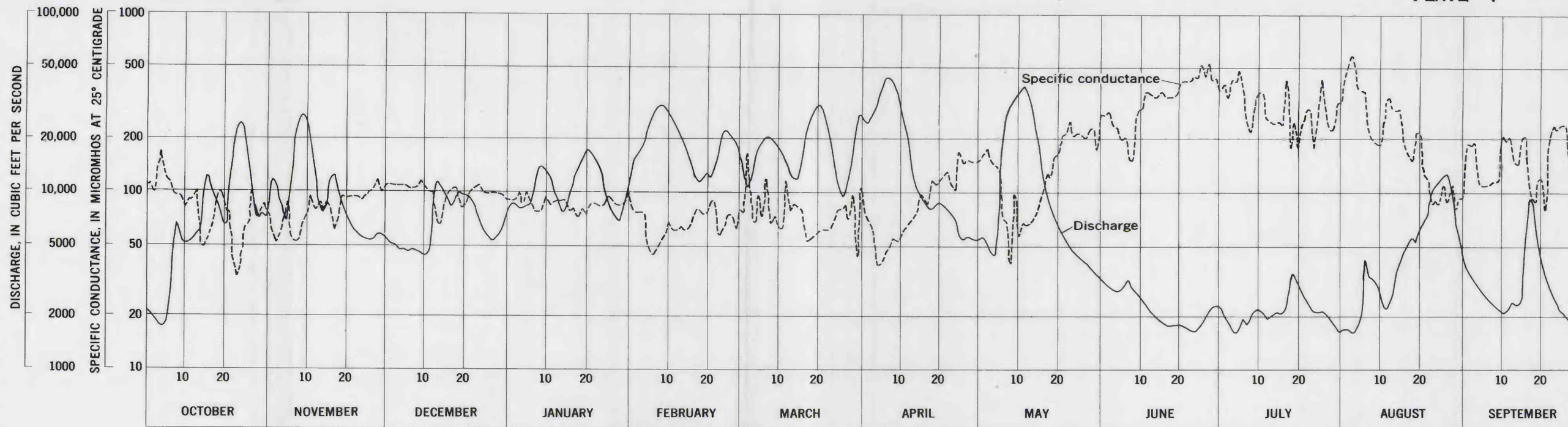
SPECIFIC CONDUCTANCE OF DAILY SAMPLES AND DAILY MEAN DISCHARGE PASCAGOULA RIVER NEAR BENNDALE, MISSISSIPPI, WATER YEAR 1960
