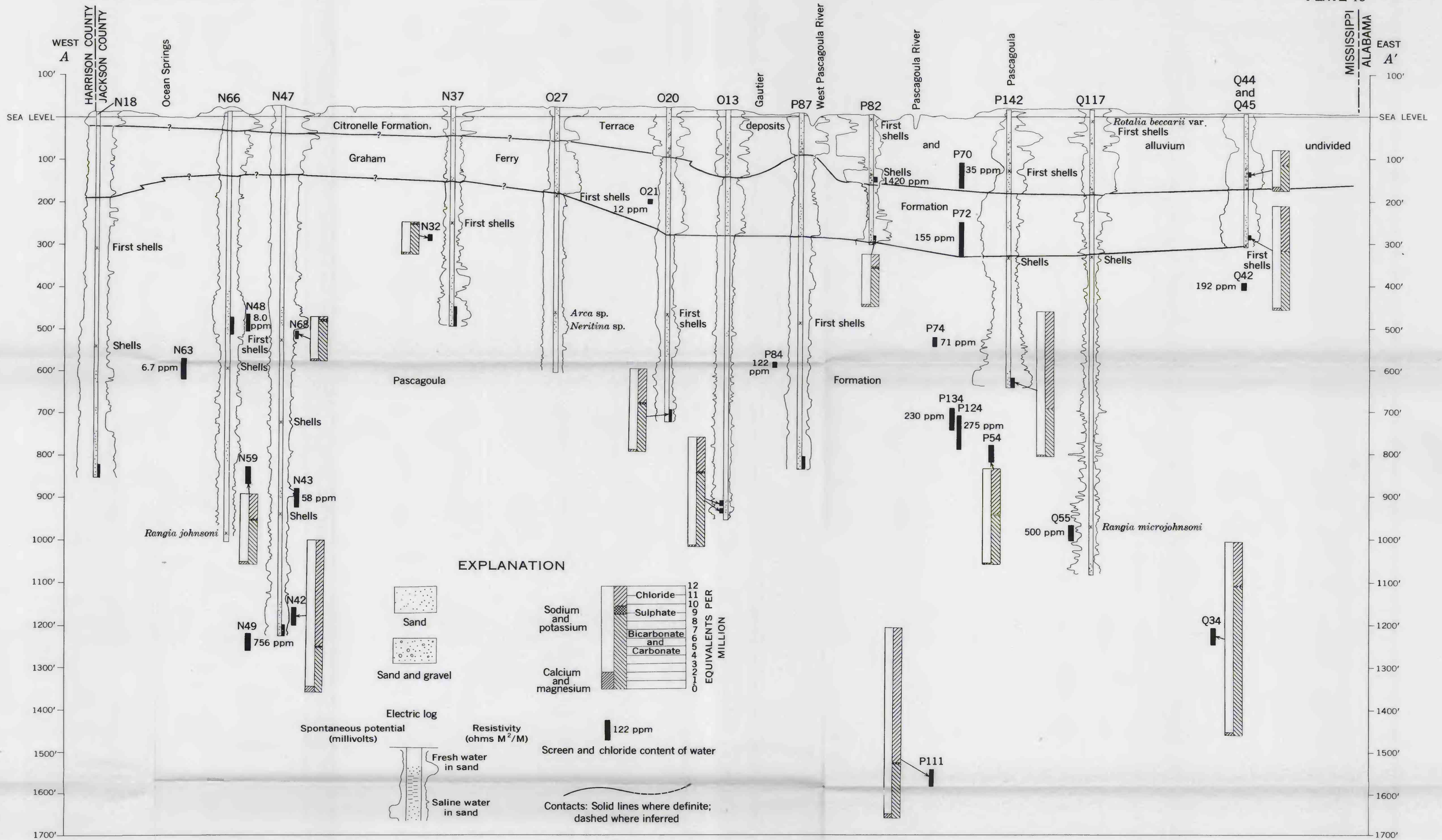
GEOLOGIC SECTION A-A' NEAR COASTLINE OF JACKSON COUNTY, MISSISSIPPI
