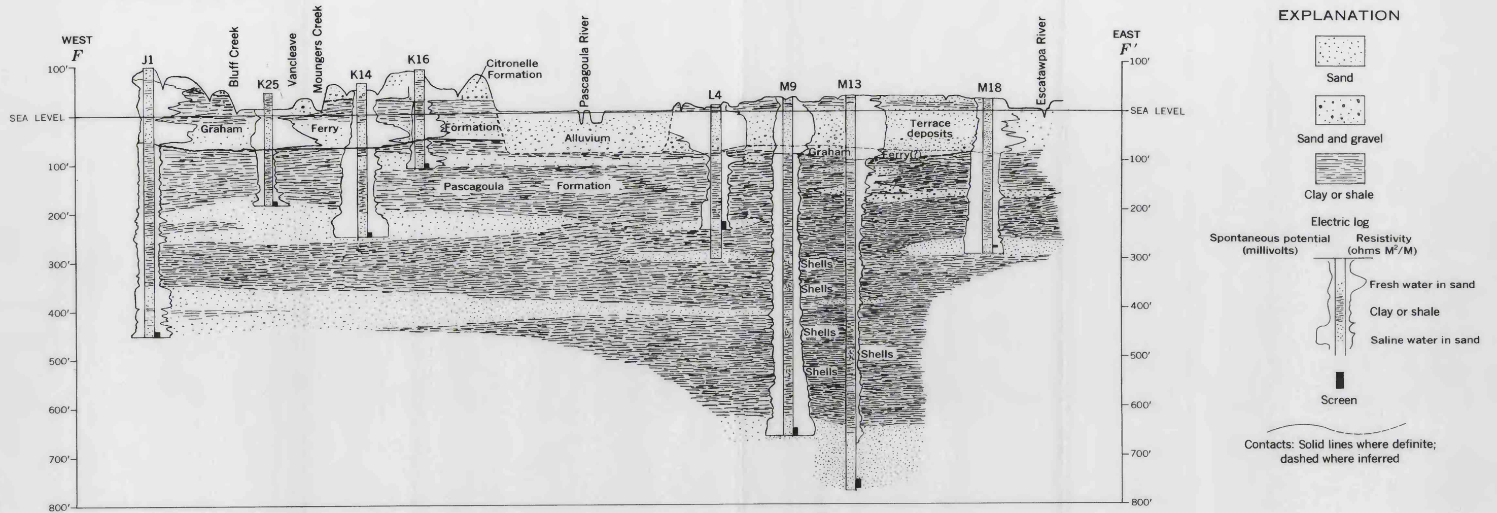
GEOLOGIC SECTION F-F' ACROSS PASCAGOULA RIVER, VANCLEAVE TO ESCATAWPA RIVER, MISSISSIPPI
