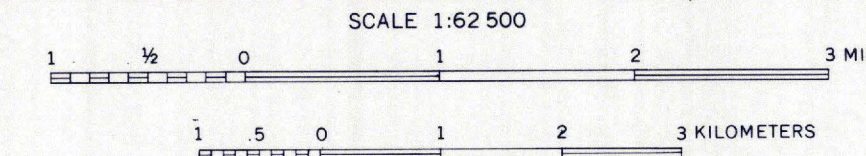
MAP OF THE BABYLON-ISLIP AREA, SHOWING GENERALIZED SURFICIAL GEOLOGY, LOCATION OF WELLS, AND GEOLOGIC SECTION A-A' FROM FIRE ISLAND STATE PARK TO BRENTWOOD, SUFFOLK COUNTY, NEW YORK
