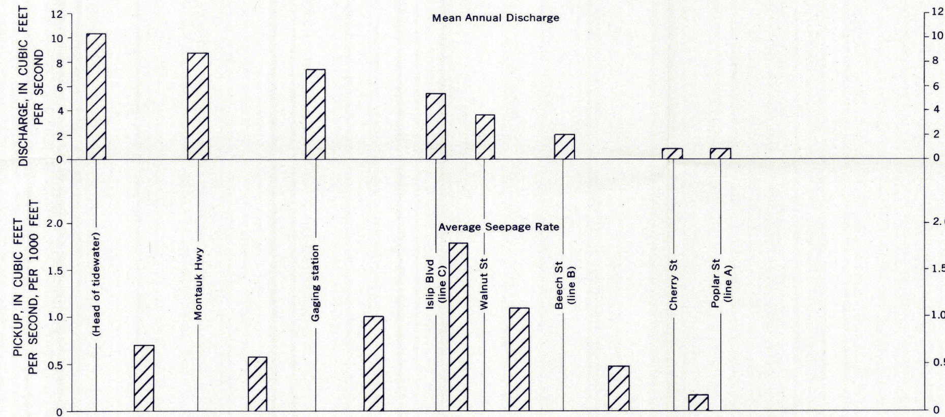
PROFILES, MEAN ANNUAL DISCHARGE AT SELECTED SITES, AND AVERAGE SEEPAGE RATES (PICKUP) OF THREE STREAMS IN THE BABYLON-ISLIP AREA, SUFFOLK COUNTY, NEW YORK
