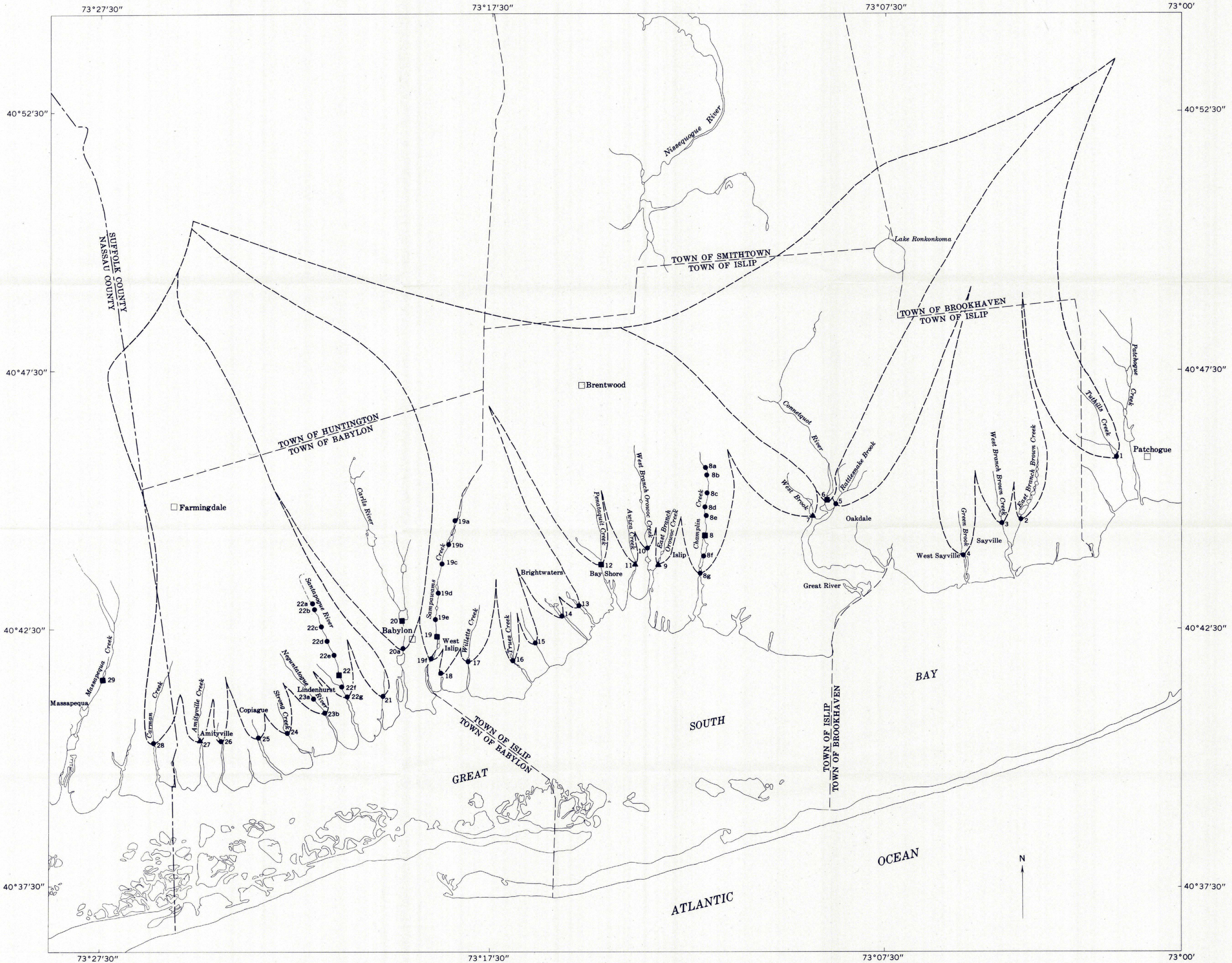
LOCATION OF STREAM-GAGING SITES AND PRECIPITATION STATIONS AND OUTLINES OF GROUND-WATER CONTRIBUTING AREA, BABYLON-ISLIP AREA, SUFFOLK COUNTY, NEW YORK
