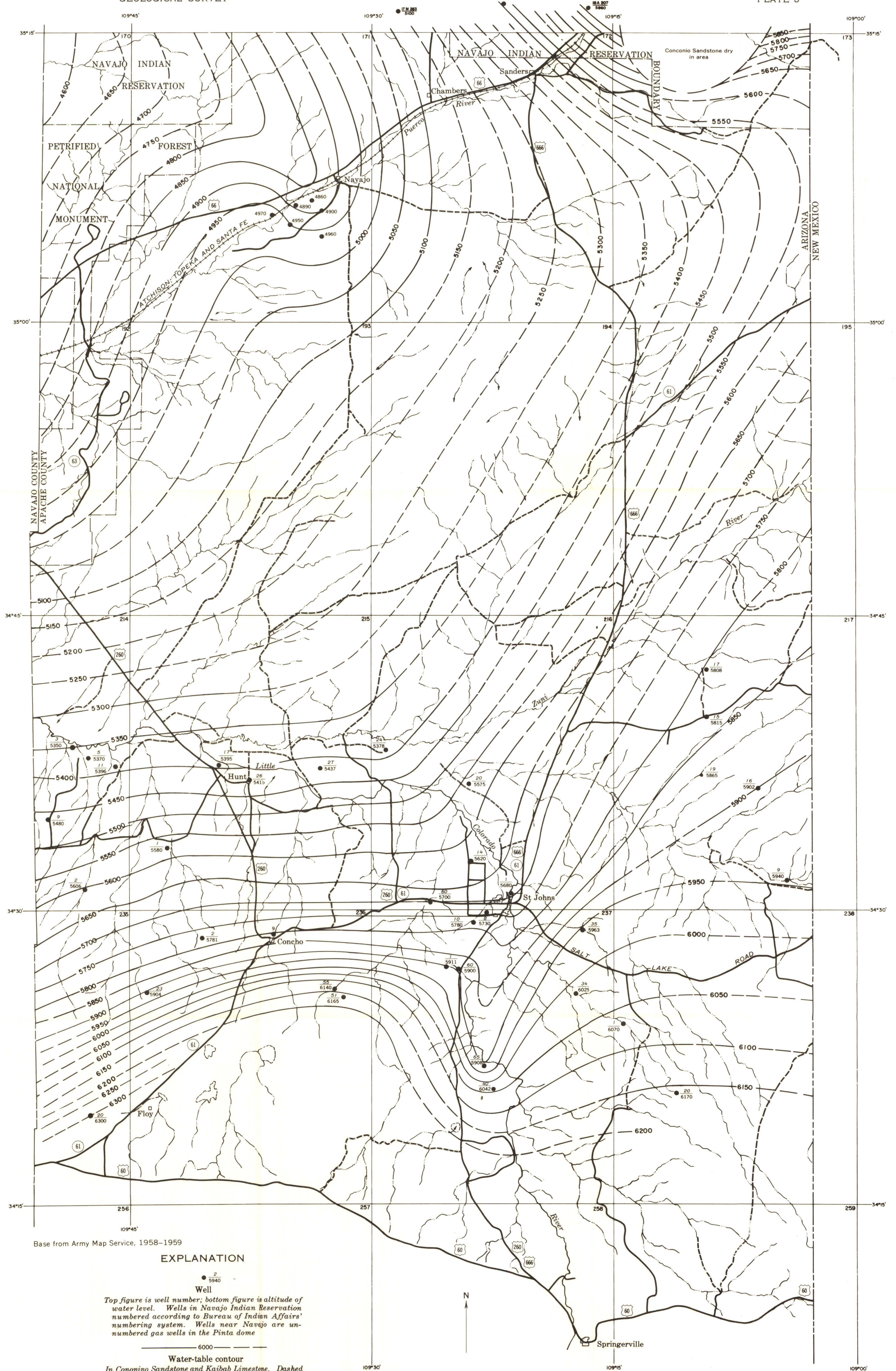
MAP SHOWING CONFIGURATION OF WATER TABLE IN THE COCONINO SANDSTONE AND KAIBAB LIMESTONE IN THE CENTRAL PART OF APACHE COUNTY, ARIZONA
