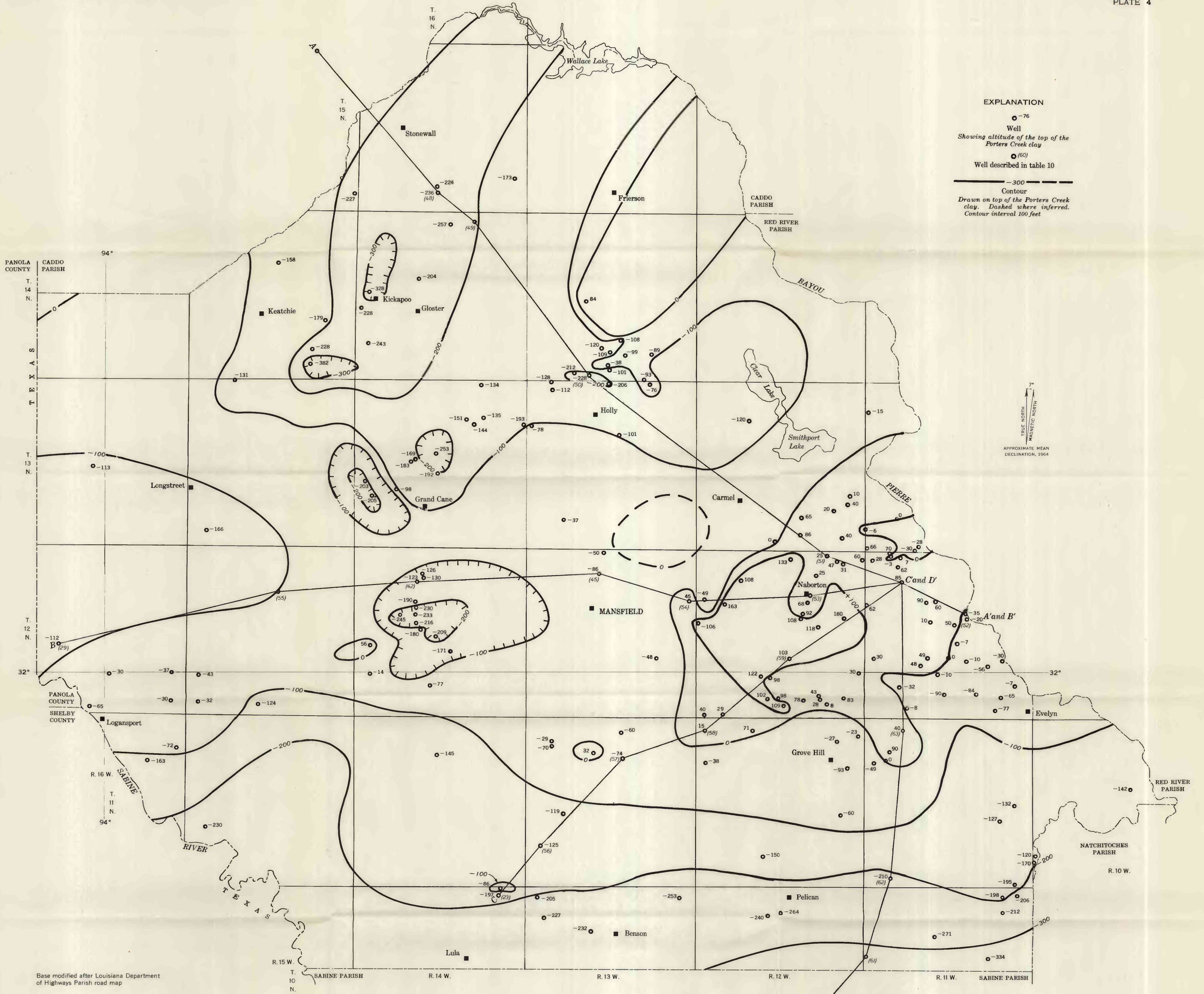
MAP OF DE SOTO PARISH SHOWING CONTOURS ON THE TOP OF THE PORTERS CREEK CLAY AND LOCATION OF GEOLOGIC SECTIONS
