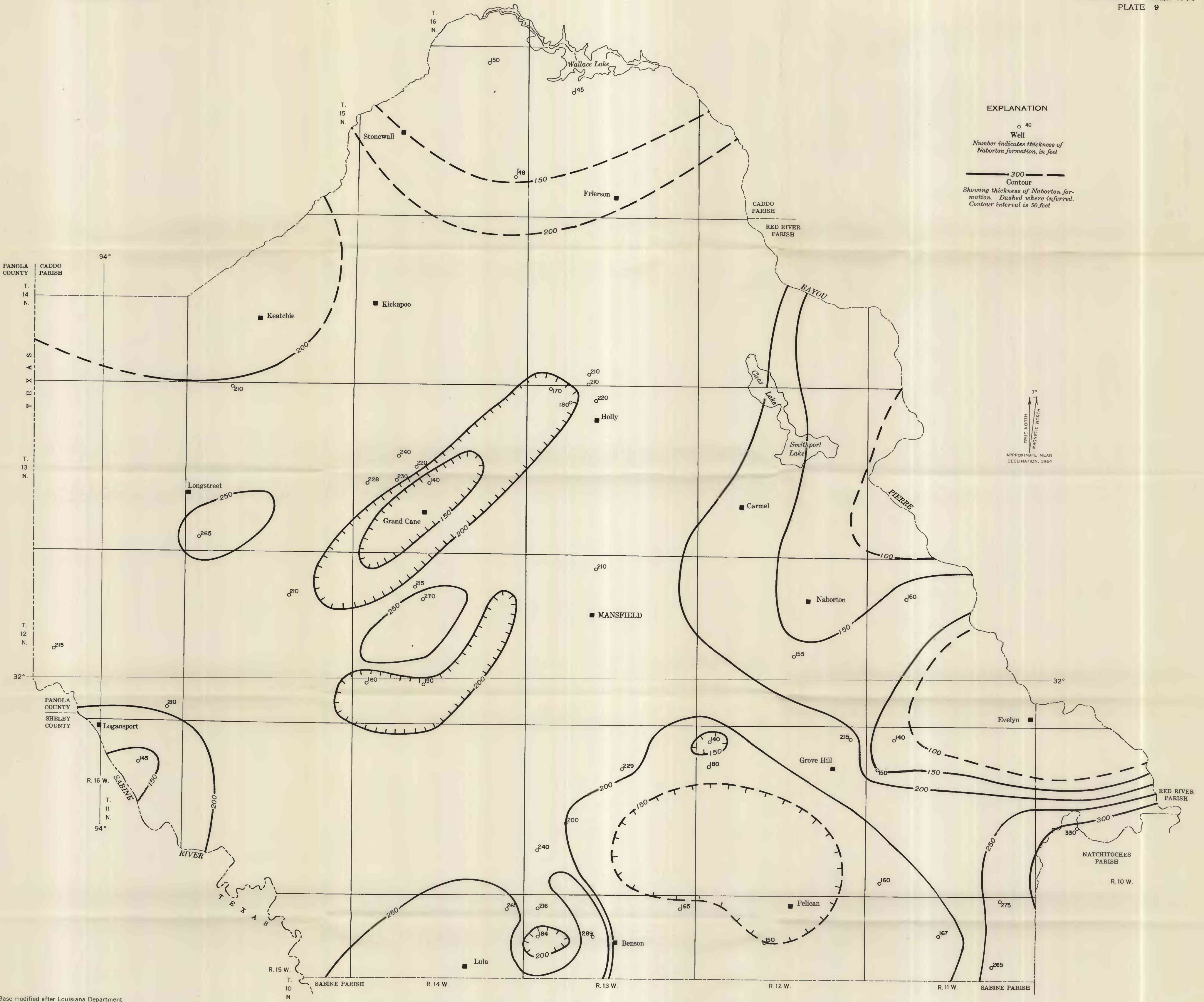
MAP OF DE SOTO PARISH, LOUISIANA, SHOWING THICKNESS OF THE NABORTON FORMATION
