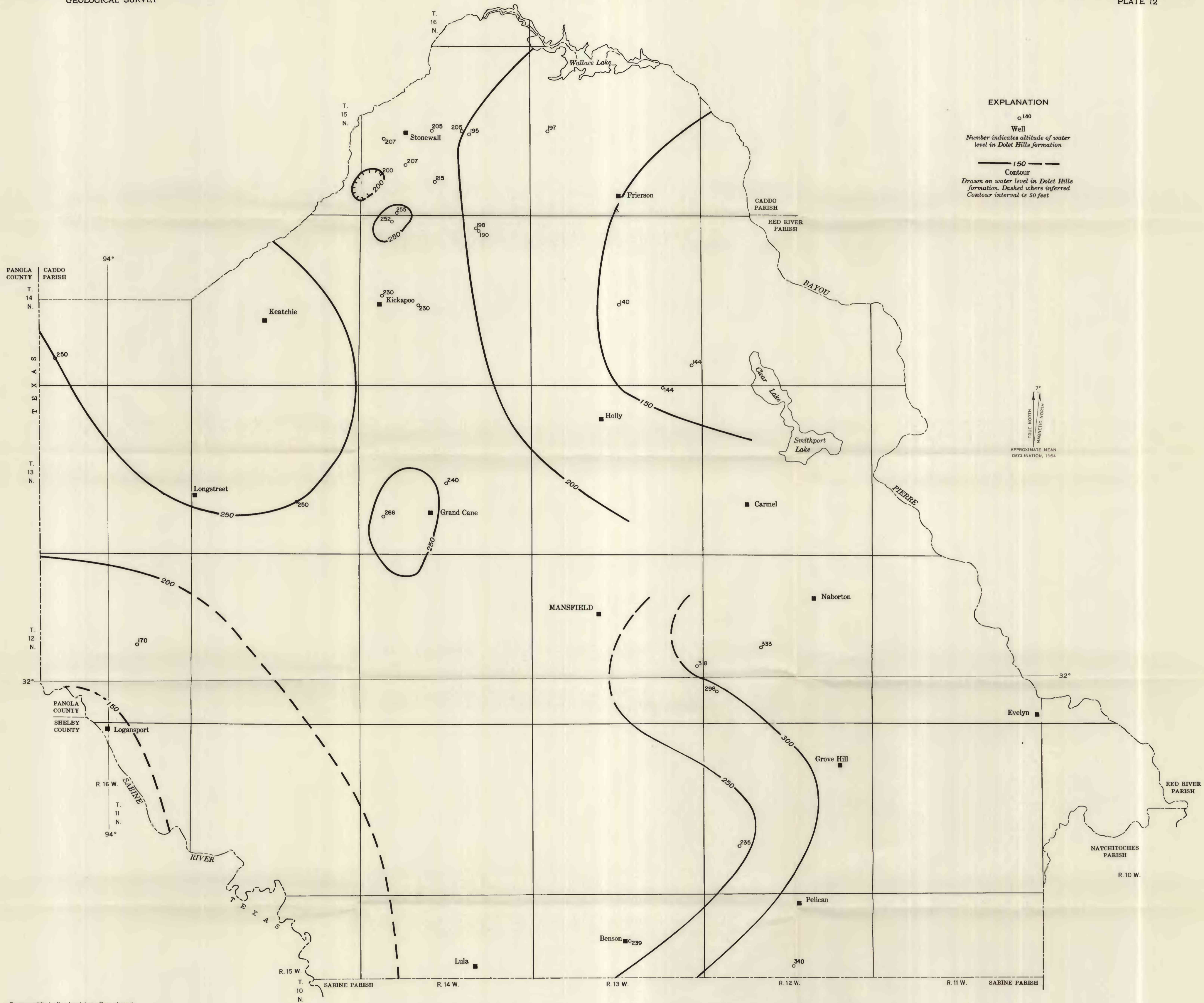
MAP OF DE SOTO PARISH, LOUISIANA, SHOWING ALTITUDE OF WATER LEVELS IN THE DOLET HILLS FORMATION
