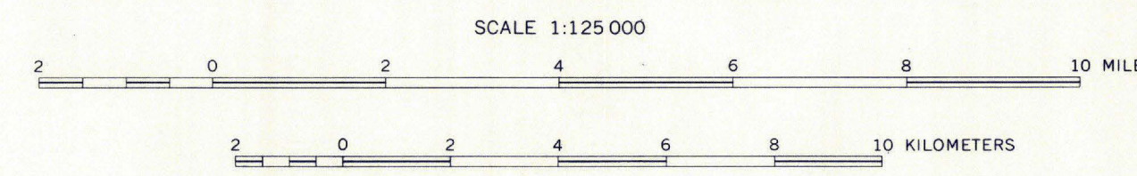
MAP SHOWING CONFIGURATION OF THE BEDROCK SURFACE BENEATH THE HIGH PLAINS PROVINCE OF WASHINGTON COUNTY, COLORADO
