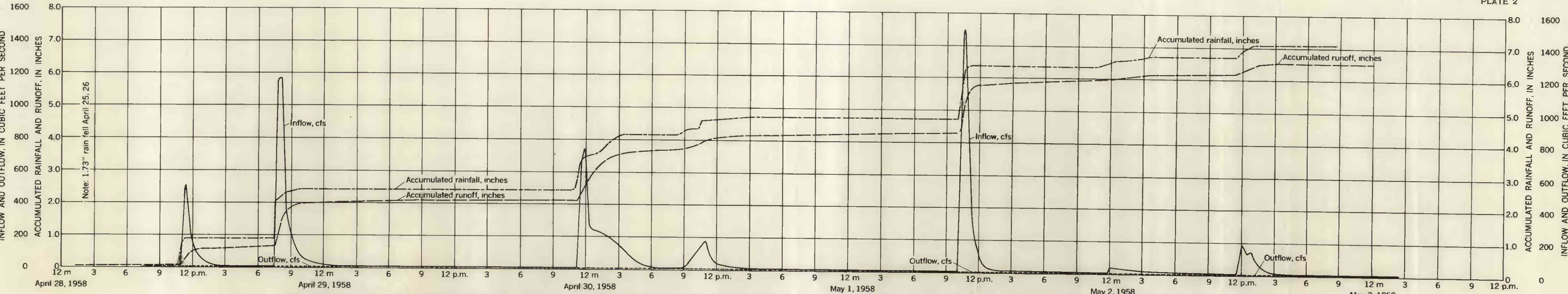
RAINFALL AND RUNOFF AT SITE 12, HONEY CREEK BASIN, TEXAS, STORM PERIOD APRIL 28 TO MAY 3, 1958
