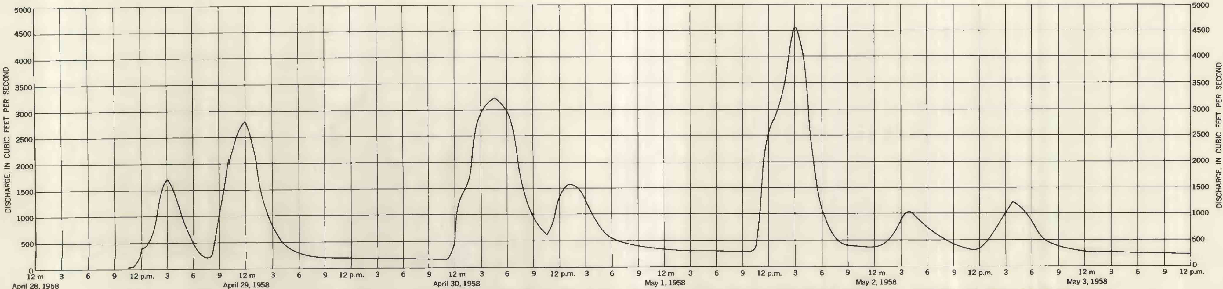
STORM HYDROGRAPH AT STREAM-GAGING STATION, HONEY CREEK NEAR MC KINNEY, TEXAS, APRIL 28 TO MAY 3, 1958
